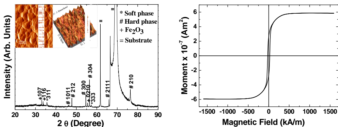
Figure 2. Composite BaFe 12 O 19 + Mg 0.1 Ni 0.3 Zn 0.6 Fe 2 O 4 thin film deposited on the Si (100) substrate, when cooled in the presence of oxygen pressure: XRD pattern (left panel), AFM 2D and 3D images (inset), and hysteresis loop (right panel).
