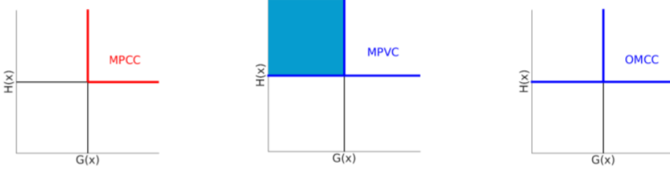
Figure 1: Feasible set of the complementarity, vanishing and kink constraint.
