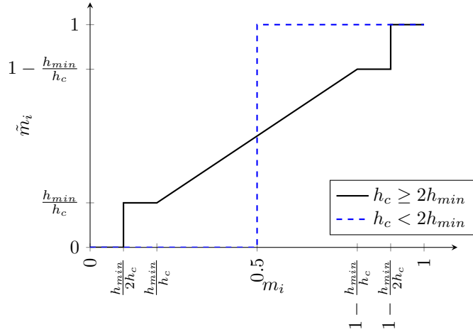
Figure 22: Thresholds for the post-treatment, or \tilde{m}_i as a function of m_i , in order to fulfill a minimal feature size h_{min}
