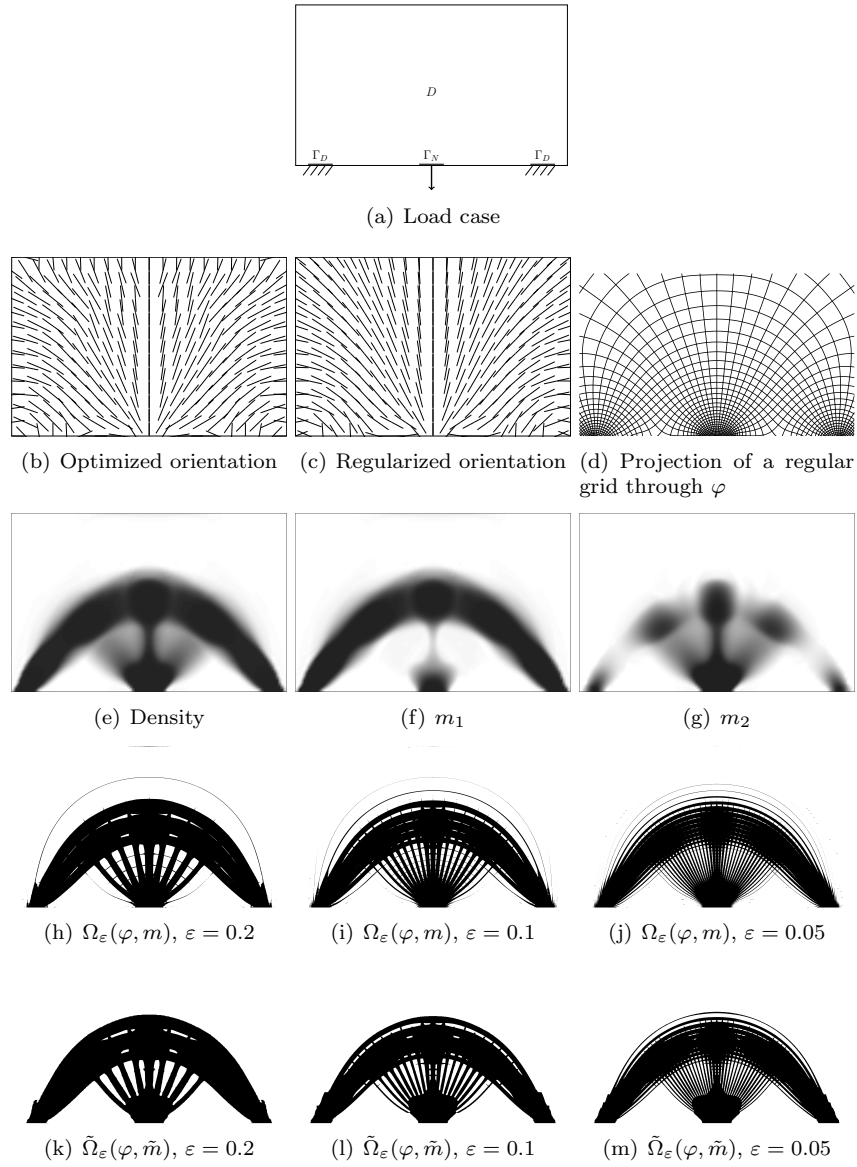
Figure 25: Complete process for an arch case
