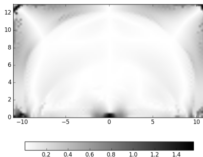
Figure 12: Angle difference in radian between the optimized orientation and the regularized orientation for the bridge case
