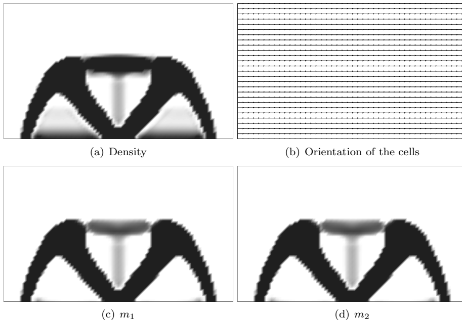
Figure 9: Optimized design of the bridge, case B : \alpha = 0 .
