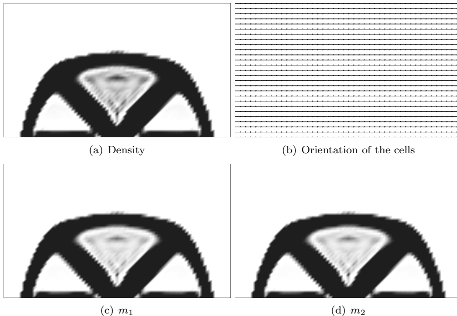
Figure 10: Optimized design of the bridge, case D : m_1 = m_2 and \alpha = 0 .
