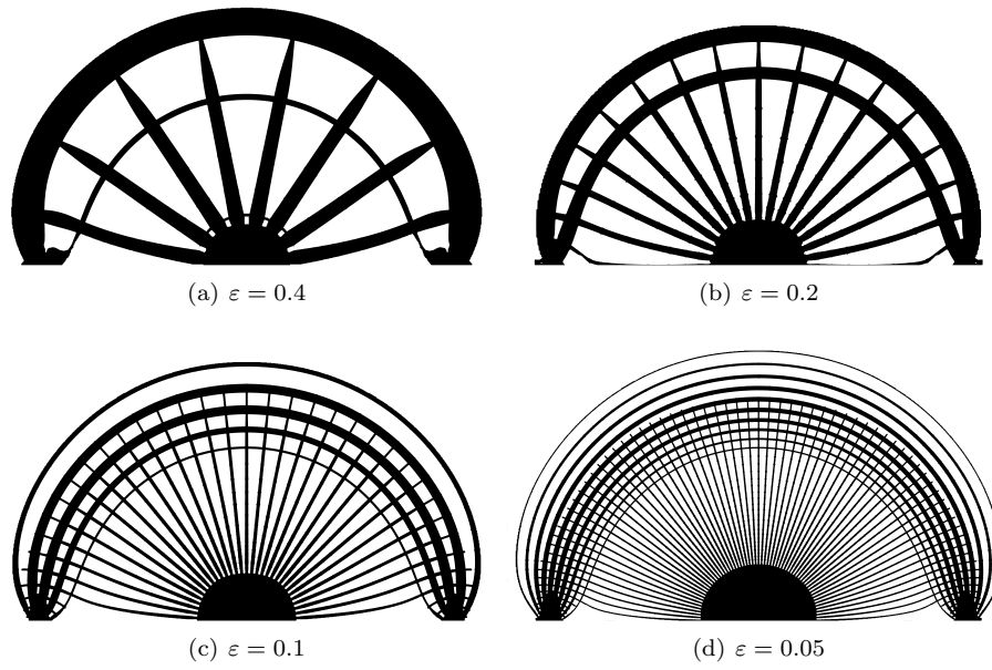
Figure 24: Post-processed structures \tilde{\Omega}_\varepsilon(\varphi, \tilde{m}) for several \varepsilon in the case of the bridge
