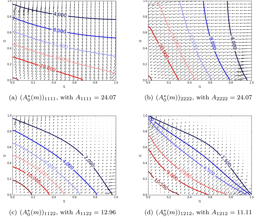
Figure 4: Isolines of the entries of the homogenized tensor A^* and their gradient (small arrows) according to the parameters m . The x -axis is m_1 , the y -axis is m_2
