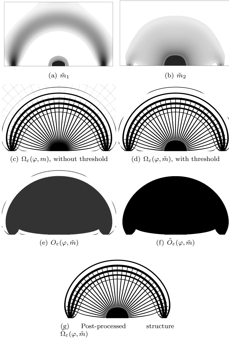
Figure 23: Results of the post-treatment for the bridge case, with a minimal feature size h_{min} = 0.05\varepsilon (here : \varepsilon = 0.1 )
