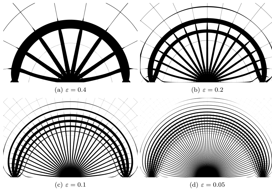
Figure 21: \Omega_\varepsilon(\varphi, m) for several \varepsilon in the case of the bridge
