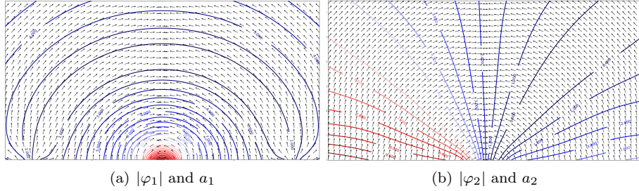
Figure 19: Map \varphi (isolines) and the vectors a_i (arrows) for the bridge case
