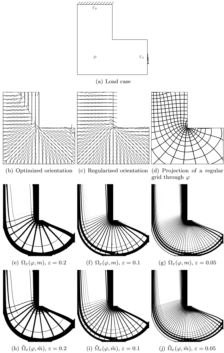
Figure 28: Complete process for a L-beam
