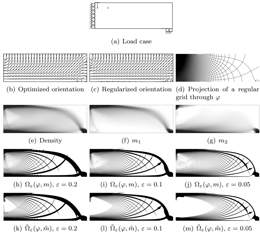
Figure 27: Complete process for a MBB beam
