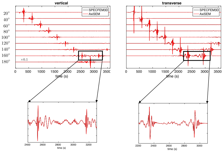
Fig. 11 Comparison of 1D numerical simulations from SPECIFEM3D_GLOBE and AxiSEM for the Sohl & Spohn model. The seismograms are filtered between 10 s and 250 s. Epicentral distances are shown on the left and antipodal seismograms are scaled by 10. Moment tensor solution of the 2011 Virginia earthquake ( M_w = 5.8 , depth = 12 km) is used as a source during simulations where the source and receivers are located along the equator
