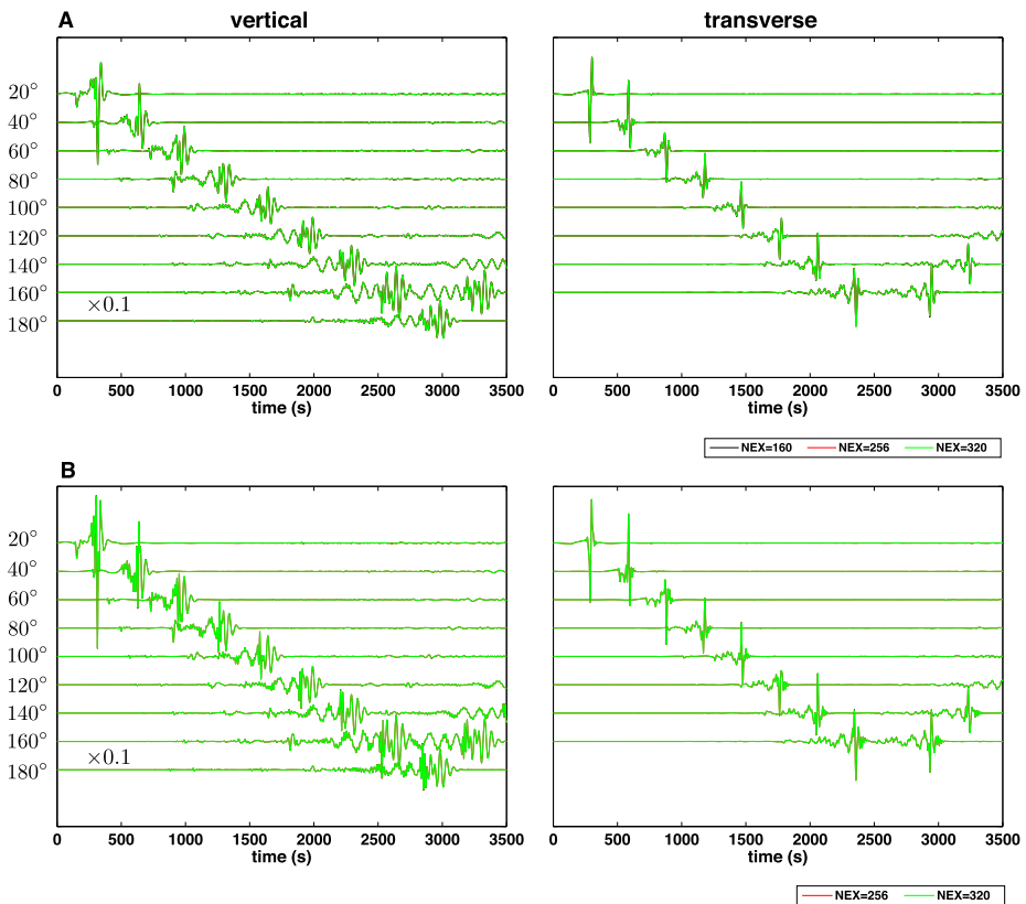
Fig. 2 Resolution of 1D simulations for various meshes with NEX = 160, 256, and 320 , where NEX is the number of spectral elements along one side of each of the six chunks that constitute the cubed sphere on the surface. Seismograms are bandpassed between (A) 20 s and 250 s, (B) 15 s and 250 s, indicating that the NEX = 160 and NEX = 256 meshes resolve waves with a shortest period down to 20 s and 15 s, respectively. Vertical- and transverse-component seismograms show P, SV & Rayleigh waves and SH & Love waves, respectively. Antipodal seismograms are normalised by 10. Moment tensor solution of the 2011 Virginia earthquake ( M_w = 5.8 , depth = 12 km) is used as a source during simulations where the source and receivers are located along the equator with 20^\circ epicentral distance spacing, as denoted on the left
