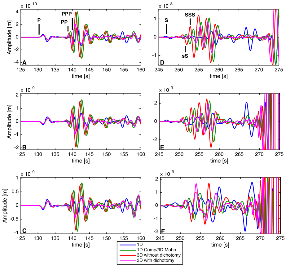
Fig. 14 Three-component (A—Radial; B—Transverse; C—Vertical) synthetic seismograms computed at an epicentral distance of 16.2° to the North-East of the event (inverted gray triangle in Fig. 12) using four different models. Model “1D” represents the one-dimensional model shown in Fig. 13E (black bold line); “1D/3D” (not shown) is a composite model consisting of a 1D crustal velocity component and a three-dimensional (3D) crustal thickness component; “3D” represent the three-dimensional models without (Fig. 13A–B) and with crustal dichotomy (Fig. 13C–D). A number of P-wave phases based on the “1D” model are indicated for reference. The mantle component underneath all models is assumed to be one-dimensional. Seismograms have been filtered between 2–100 s using a third-order Butterworth filter. The event is a double-couple ( M_w = 2.98 ) located at a depth of 3 km
