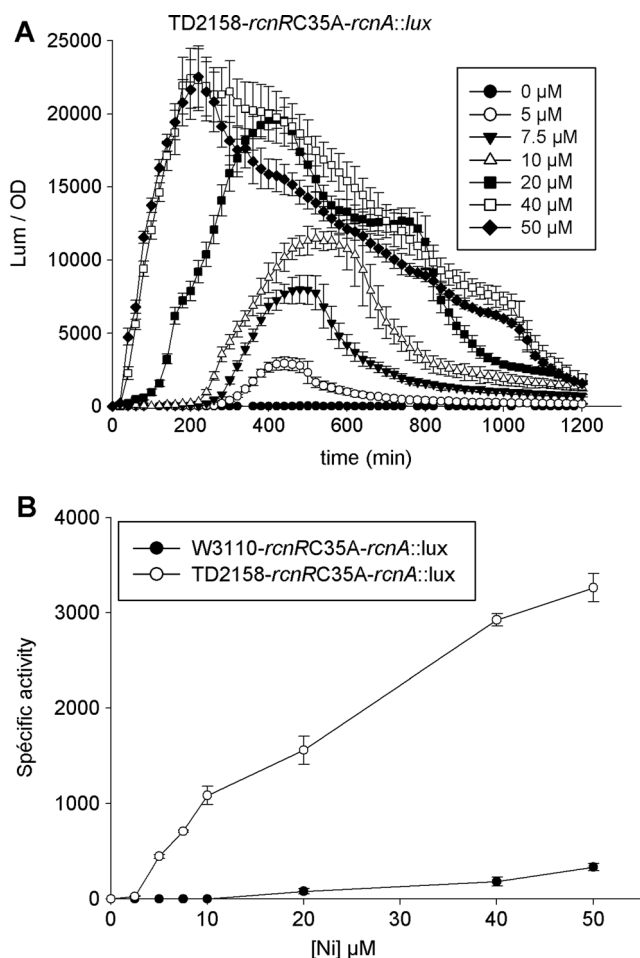
Fig. 6 The detection of Ni is influenced by the genetic background. a Kinetics response of the TDRAlux strain grown in the presence of increasing \text{NiCl}_2 concentration. The luminescence was recorded during 20 h; the activity is presented on the graph (luminescence (A.U.)/OD 600 nm ). The experiments were repeated at least three times; SD are presented on the graph. b Comparison of two E. coli sensor strains. TDRAlux strain and WC35Alux strain were grown in the presence of increasing concentrations of Ni. The luminescence was recorded during 16 h. The value of the maximum specific activity is plotted on the graph (luminescence (A.U.)/OD 600 nm /time (min)). The experiments were repeated at least three times; SD are presented on the graph
