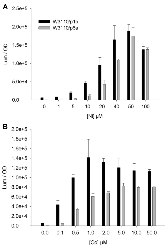
Fig. 1 Response of the PrcnA::lux fusion. W3110 (WT) strain containing plasmids p1b ( P rcnA ::lux ) (black) or p6a ( rcnR- P rcnA ::lux ) (grey) was grown in the presence of a NiCl 2 or b CoCl 2 . The luminescence was recorded during 8 h; the value of the maximum activity is plotted on the graph (luminescence (A.U.)/OD 600 nm ). The experiments were repeated at least three times; SD are presented on the graph
