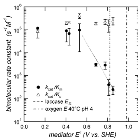
Figure 11. Effect of mediator redox potential, E^0 , on laccase-mediator bimolecular rate constant, k_{cat}/K_m , and laccase-oxygen rate constant, k_{cat}/K_s . Also shown are redox potentials of laccase and O_2/H_2O at pH 4. A linear free energy region is observed for high E^0 (small \Delta E_{ct} ) and constant mediation rate at lower E^0 values. Reproduced with permission from [190]. Copyright 2008 American Chemical Society.
