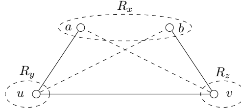
Fig. 2: A broken triangle (a, u, v, b) having a and b as end points. Inconsistent values are related by a dashed edges.
