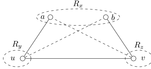
Fig. 2: A broken triangle (a, u, v, b) having a and b as end points. Inconsistent values are related by a dashed edges.
