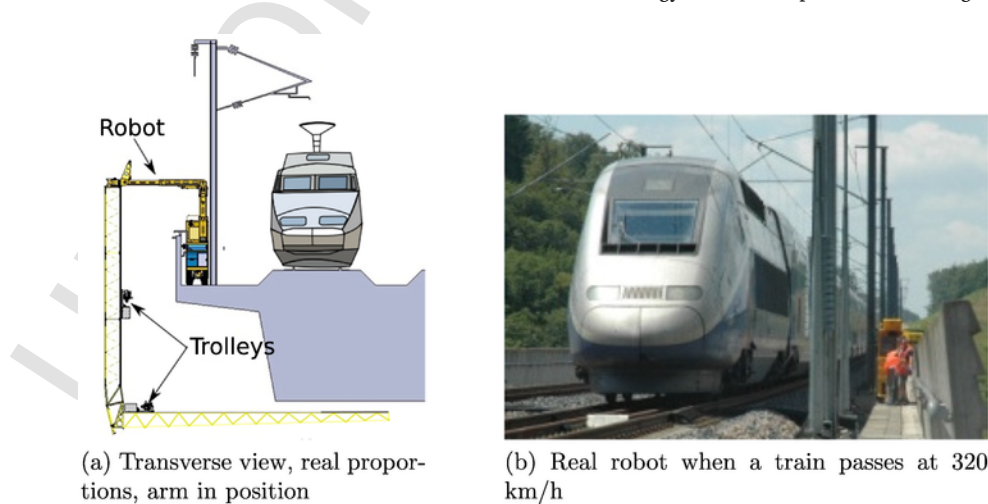
Fig. 3. Mobile robot on a high speed train bridge.
