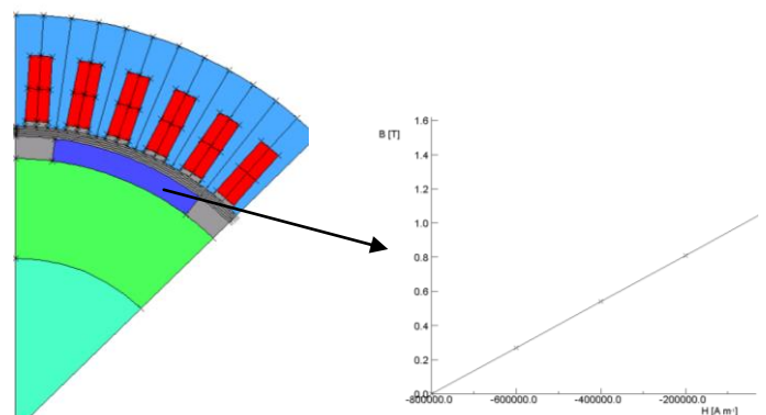
Figure 1. 1/8 of synchronous machine with magnet characteristic
