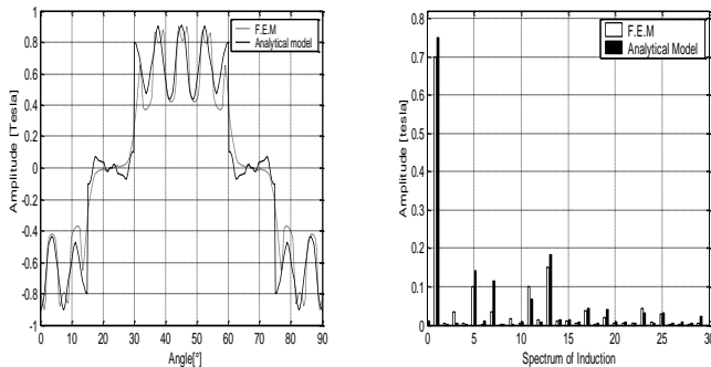
Figure 2. Comparison of the form induction and FFT
