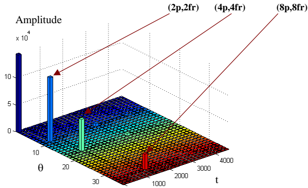
Figure 3. FFT 2D of radial force (fr = p×N)
