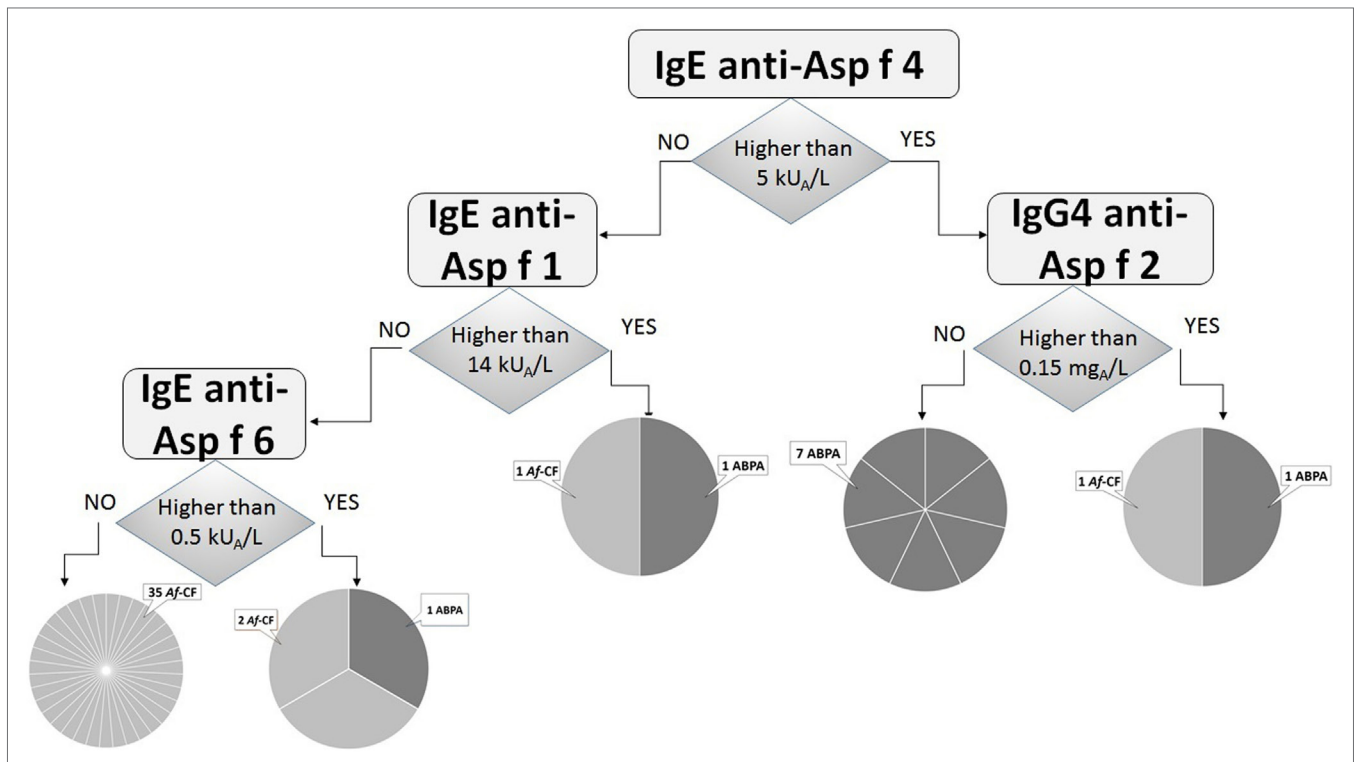
FIGURE 2 | Classification tree using analysis of sIgE, sIgG, and sIgG4 responses to Asp f 1, Asp f 2, Asp f 3, Asp f 4, and Asp f 6 molecules. The diagnostic algorithm retains IgE to Asp f 4, Asp f 1, Asp f 6, and IgG4 to Asp f 2, yielding 1 Aspergillus fumigatus ( Af )-cystic fibrosis (CF)-only groups counting 35/39 patients, 1 allergic bronchopulmonary aspergillosis (ABPA)-only group of 7 patients, and 3 mixed groups of undetermined clinical significance where other criteria are needed. Overall, 7/10 ABPA patients and 35/39 Af -CF patients are clearly identified.
