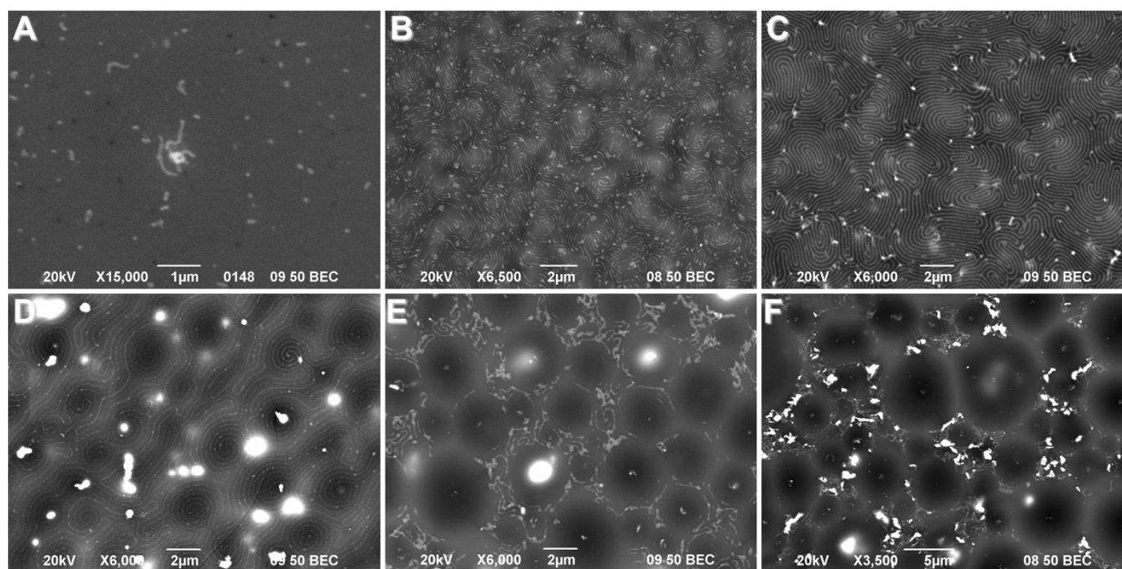
Fig. 4. Sequence of cholesteric patterns of gold nanoparticles when the thickness increases (SEM, backscattered electrons mode). Two thickness regimes are described. Thickness < 2 \mu\text{m} : (A) nuclei, (B) fingers, (C) fingerprint texture. Thickness > 2 \mu\text{m} : (D) double-spiral network (thickness range was 2 to 12 \mu\text{m} ), (E) targets (thickness range was 12 to 25 \mu\text{m} ), (F) aggregates (thickness > 25 \mu\text{m} ).
