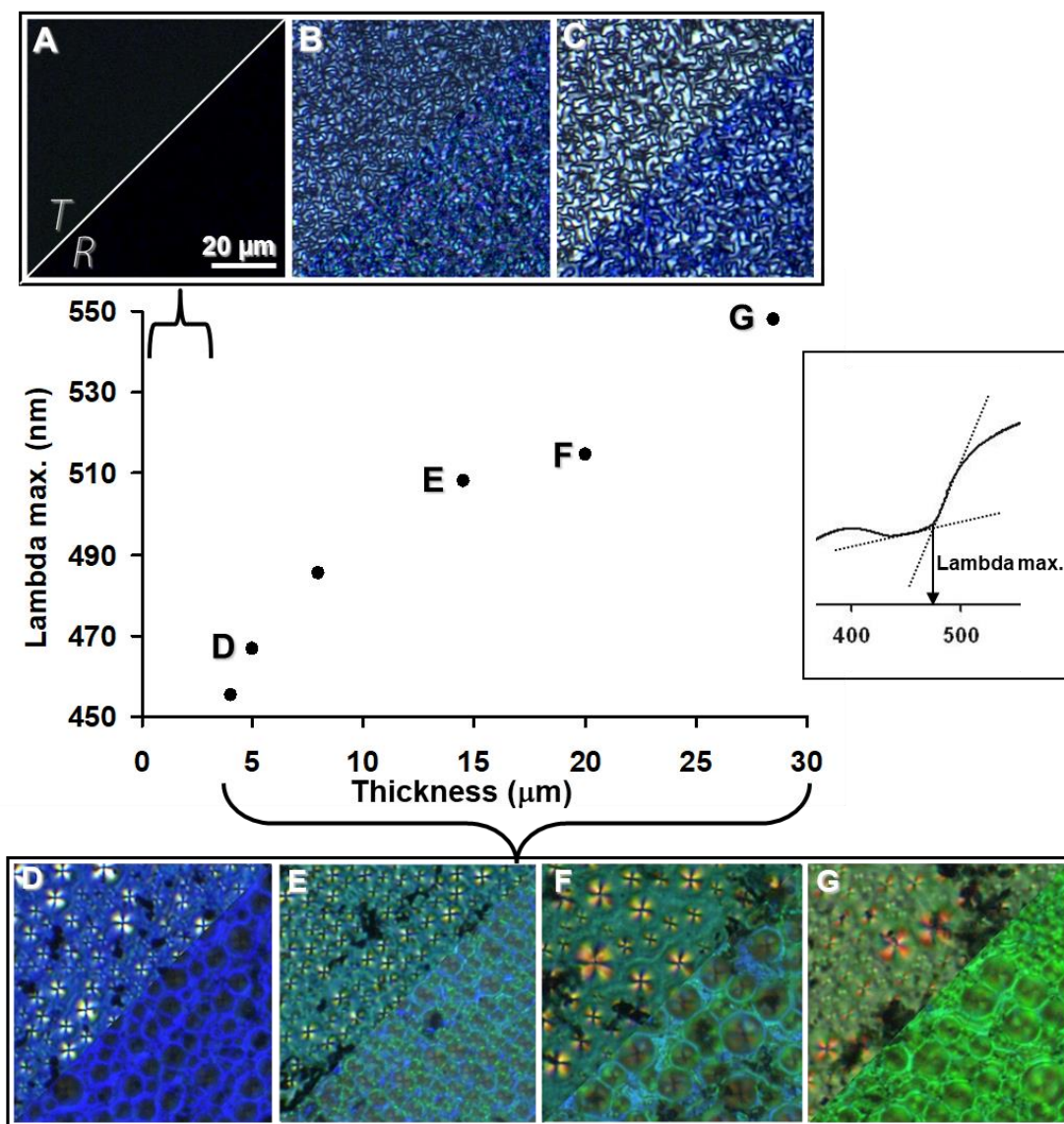
Fig. 10. Reflection wavelength as function of film thickness (unpolarized incident light). The wavelength ( \lambda_{\text{max}} ) is the right-edge value of the band-gap plateau (as shown in the inserted drawing). Inset shows optical textures (crossed polarizers) in transmission ( T ) and reflection ( R ) modes for increasing film thickness. Images A, B, and C ( resp. D to G) correspond to thicknesses < 2 \mu\text{m} ( resp. between 5 and 30 \mu\text{m} ).
