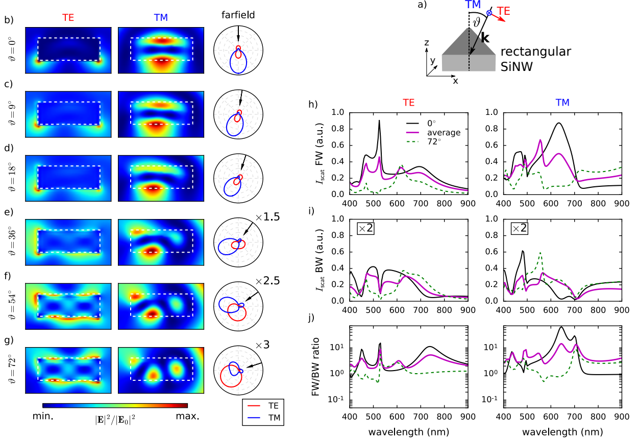
FIG. 6. (a) sketch illustrating the oblique incident illumination. (b-g) Electric field intensities (individually normalized) in the cross section of rectangular SiNWs of width W = 250 nm (height H = 90 nm) for increasing incident angles from normal incidence in (b) to \vartheta = 72^\circ in (g). The NW cross section is indicated by dashed white lines. Left: TE, center: TM polarized plane wave of wavelength \lambda_0 = 600 nm. Right: farfield pattern for TE (red) and TM (blue). In the farfield panels, the corresponding angle of incidence is depicted by a black arrow. (h-j) show corresponding farfield spectra for TE (left) and TM (right) polarization. (h) forward scattering (towards lower hemisphere), (i) backward scattering (to upper hemisphere, multiplied by 2) and (j) FW/BW scattering ratio for normal incidence (black lines), averaged incident angles from 0^\circ to 72^\circ (magenta lines) and 72^\circ (green dashed lines). 72^\circ corresponds to the maximum angle of the darkfield illumination in our experiments.
