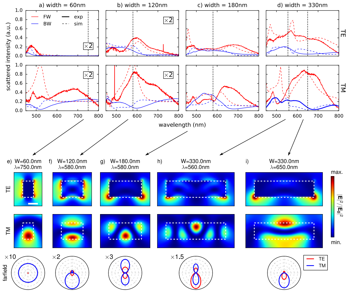
FIG. 5. (a-d) selected scattering spectra from rectangular silicon nanowires. Experimental FW (red) and BW (blue) scattered intensity (solid lines) is compared to GDM simulations (dashed lines) for TE (top row) and TM (bottom row) polarized plane wave illumination. NW height and length are fixed ( H = 90 nm, L = 7 \mu m), widths W are (a) 60 nm, (b) 120 nm, (c) 180 nm and (d) 330 nm, referring to the simulation parameters. Intensities in (a-b) are multiplied by \times 2 for better visibility. Same data as in figure 4. Panels (e-i) show selected electric field intensities in the cross section of rectangular SiNWs for (e) W = 60 nm, \lambda = 750.0 nm; (f) W = 120.0 nm, \lambda = 580.0 nm; (g) W = 180.0 nm, \lambda = 580.0 nm; (h) W = 330.0 nm, \lambda = 560.0 nm and (i) W = 330.0 nm, \lambda = 650.0 nm. Plane wave illumination from the top, polarized perpendicularly (TE, top row) or along the NW axis (TM, bottom row). Farfield radiation patterns are shown in the bottom row (TE: red, TM: blue), adjusted by a variable scaling factor for better visibility (factor indicated on the upper left of each plot). Scale bar in (e) is 50 nm, same scale for all field plots. Vertical dashed lines in (a-d) indicate the spectral positions of the field-plots in (e-i).
