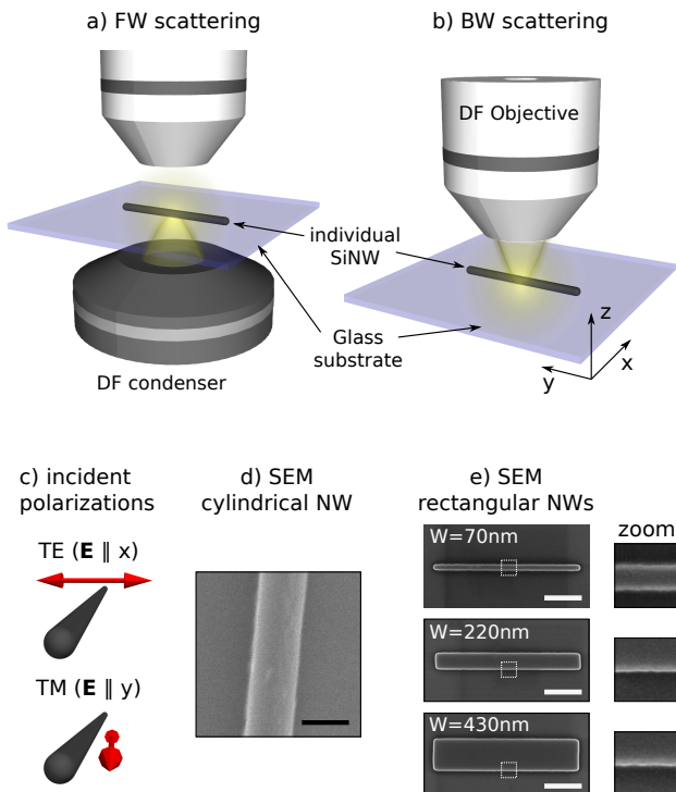
FIG. 2. Illustration of the experimental setup for (a) forward scattering and (b) backward scattering measurements. (c) sketch of the incident polarization configurations. The electric field is orientated either perpendicular (TE) or parallel (TM) to the NW axis. (d) SEM image of a cylindrical SiNW, deposited on a silicon substrate. The NWs for the spectroscopy experiments were deposited on a glass substrate, which could not be imaged in SEM due to charging. Scale bar is 100 nm. (e) SEM images of rectangular SiNWs. SEM images are obtained from a second sample on silicon on insulator (SOI) substrate. The spectroscopy sample is fabricated on transparent, but insulating SOQ substrate. Scale bars are 500 nm. Zoomed insets on the right are 200 \times 200 \text{ nm}^2 (white dashed squares indicate zoom area).
