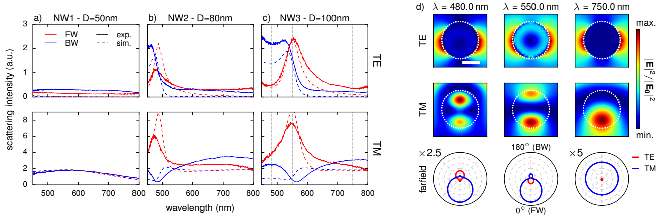
FIG. 3. Experimental (solid lines) and simulated (dashed lines) FW/BW scattering spectra (red/blue) from cylindrical NWs of different diameters. (a) D \approx 50 nm, (b) D \approx 80 nm and (c) D \approx 100 nm. Diameters are estimates by comparison to simulations. Top row and bottom row show the case of TE and TM polarized incident plane waves, respectively. (d) calculated nearfield distributions (top row: TE, center row: TM incidence) and farfield patterns (bottom row; TE/TM: red/blue) for a nanowire of D = 100 nm diameter at selected wavelengths, indicated by dashed vertical lines in (c). Plane wave incident from the top. Scale bar is 50 nm.
