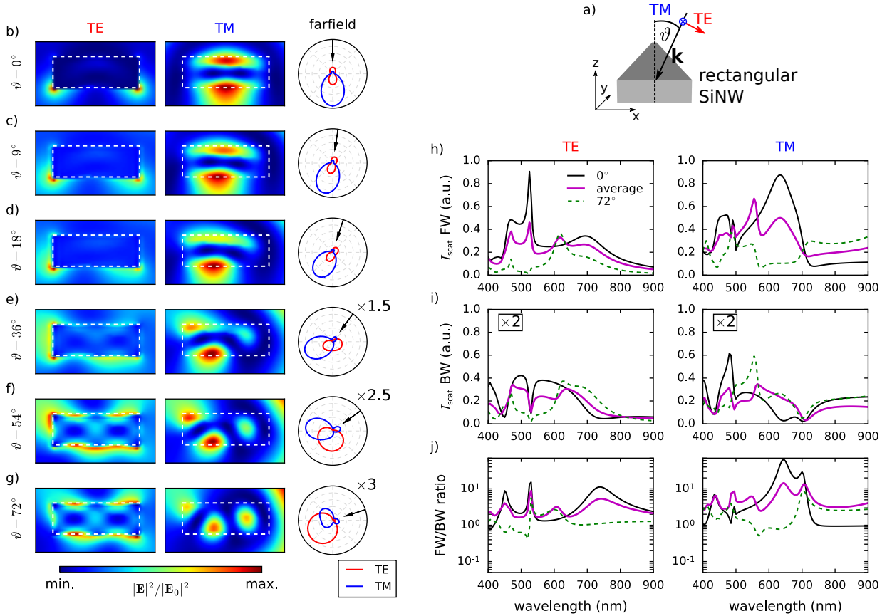
FIG. 6. (a) sketch illustrating the oblique incident illumination. (b-g) Electric field intensities (individually normalized) in the cross section of rectangular SiNWs of width W = 250 nm (height H = 90 nm) for increasing incident angles from normal incidence in (b) to \vartheta = 72^\circ in (g). The NW cross section is indicated by dashed white lines. Left: TE, center: TM polarized plane wave of wavelength \lambda_0 = 600 nm. Right: farfield pattern for TE (red) and TM (blue). In the farfield panels, the corresponding angle of incidence is depicted by a black arrow. (h-j) show corresponding farfield spectra for TE (left) and TM (right) polarization. (h) forward scattering (towards lower hemisphere), (i) backward scattering (to upper hemisphere, multiplied by 2) and (j) FW/BW scattering ratio for normal incidence (black lines), averaged incident angles from 0^\circ to 72^\circ (magenta lines) and 72^\circ (green dashed lines). 72^\circ corresponds to the maximum angle of the darkfield illumination in our experiments.
