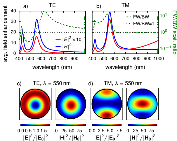
FIG. 1. Average electric (red lines) and magnetic (blue lines) field intensity enhancement inside a silicon nanowire of diameter D = 100 nm as function of wavelength for a) a TE and b) a TM polarized incident plane wave, calculated using Mie theory. Normalized to the illumination field intensity. For comparison, the FW/BW scattering ratio in the far-field is shown as dashed green line (right axis ticks). c) and d) show the internal field intensity distributions at \lambda = 550 nm for TE and TM polarization, respectively (left subplot: electric, right: magnetic field). D = 100 nm, plane wave incident from the top.
