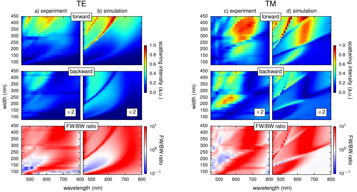
FIG. 4. Forward (top row) and backward (center row, multiplied by \times 2 for better contrast) scattering intensity from rectangular silicon nanowires as function of wavelength and NW width. Data is normalized to the global maximum intensity in FW and BW spectra. FW/BW ratios are shown in the bottom row on a logarithmic color scale. (a-b) TE, (c-d) TM polarized illumination. (a) and (c) show measured dark field spectra, (b) and (d) corresponding GDM simulations. Fixed NW height and length ( H = 90 nm, L = 7 \mu m).
