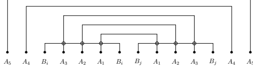
FIGURE 2. The only partition with non-zero contribution in (9) (here, k = 4, n = 6 ).
