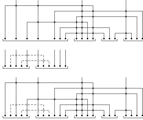
FIGURE 4. Construction of \pi (third line) from \pi_1 (second line) and \pi_2 (first line).
