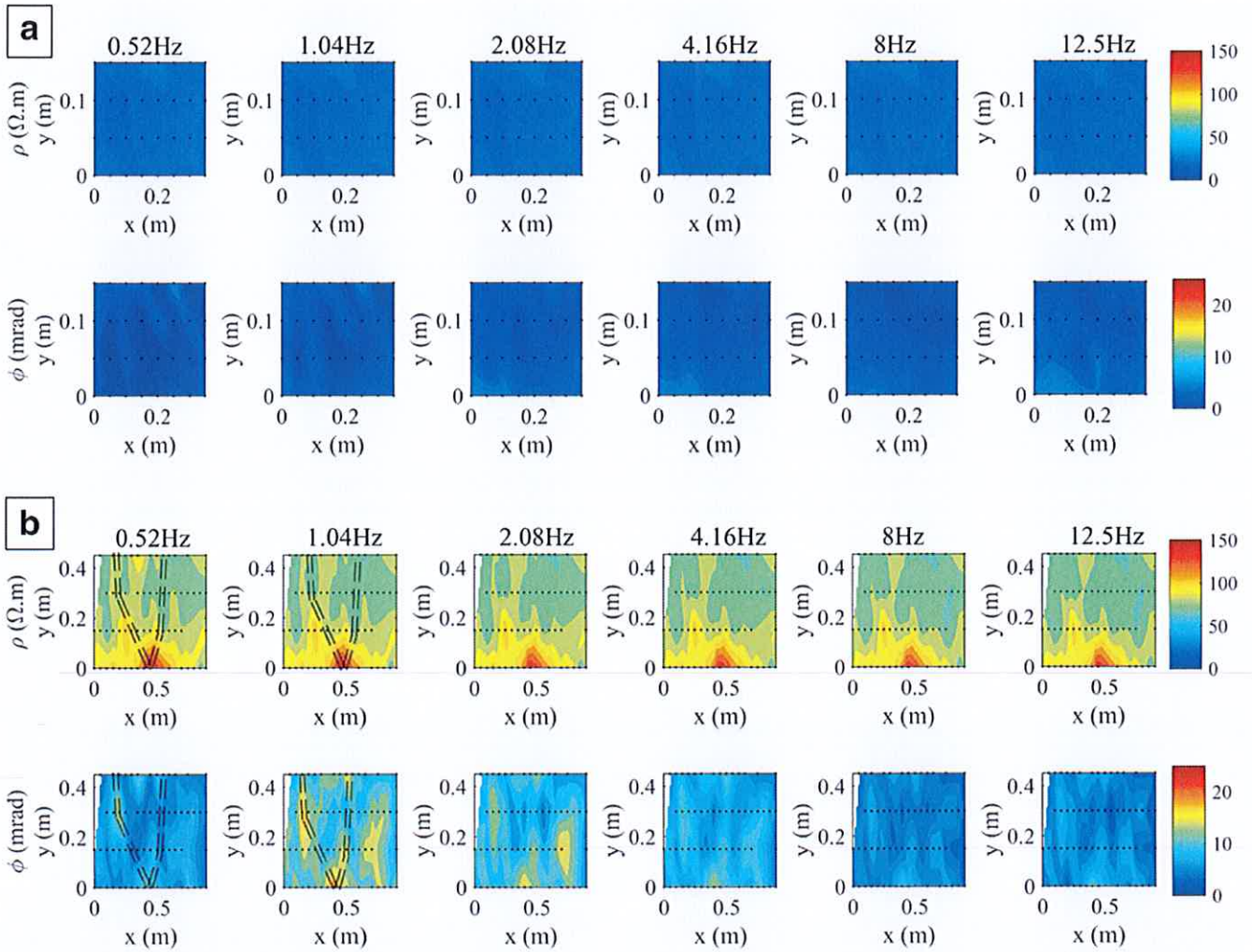
Fig. 8 Result of the SIP map produced using the LIPPMANN device a on the reference plot with the soil alone b on a plot with the study tree. For each of them, the 1st line corresponds to the
