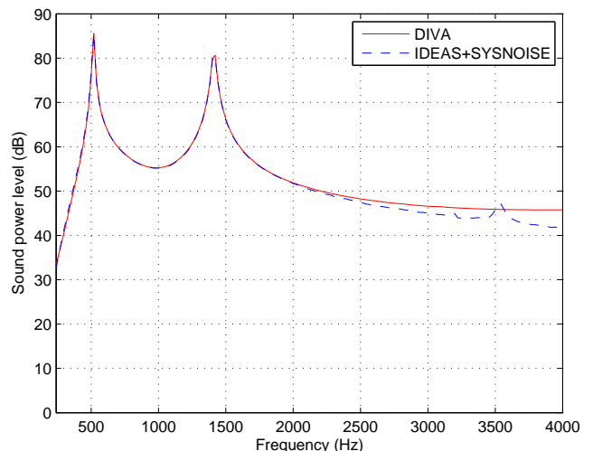
Fig. 9. Sysnoise and DIVA sound power level of a cylindrical shell submitted to two force waves of spatial order 2 and 3 rotating at variable speed.
