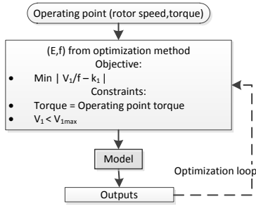
Fig. 4. Optimization method to get V_1/f=k_1
