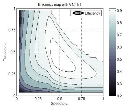
Fig. 7. Efficiency map with “ V_1/f=k_1 ” strategy
