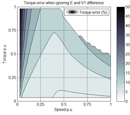
Fig. 3. Torque error in % when neglecting E and V1 difference
