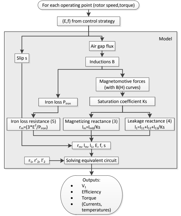
Fig. 2. Model flow chart
