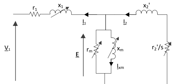
Fig. 1. Induction machine equivalent circuit
