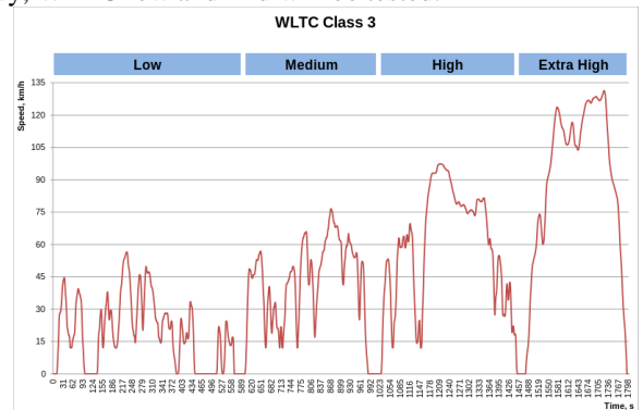
Fig. 16. WLTC driving cycle for class 3 vehicles
