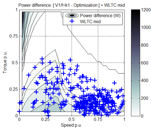
Fig. 18. Power comparison + WLTC mid operating points
