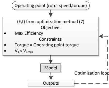
Fig. 6. Optimization strategy flow chart
