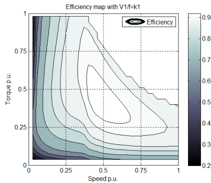
Fig. 7. Efficiency map with “ V_1/f=k_1 ” strategy
