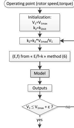
Fig. 5. “ E/f=k_2 ” strategy flow chart
