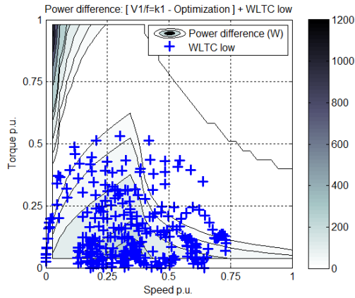
Fig. 17. Power comparison + WLTC low operating points
