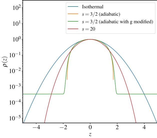
Figure 1. Density equilibrium profiles used in Sections 3 and 4, serving as a background support for the spiral density waves. The green curve corresponds to an adiabatic profile with a modified gravity so that the density converges towards a small constant value at large z . It is used in order to avoid a density floor in the adiabatic simulations of Section 4.
