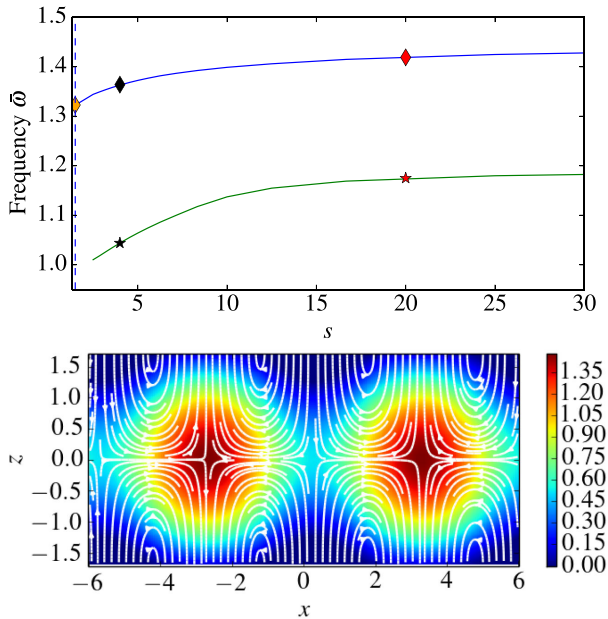
Figure 2. Top: Frequencies of the fundamental axisymmetric p mode and g mode ( n = 0 ) as a function of the polytropic index s and for k_x = (\pi/3)H_0^{-1} . Bottom: Density and poloidal streamlines of the fundamental axisymmetric p mode in an adiabatic atmosphere ( s = 3/2 ) for the same k_x . The density shown here is \rho_e + 0.6\hat{\rho} .
