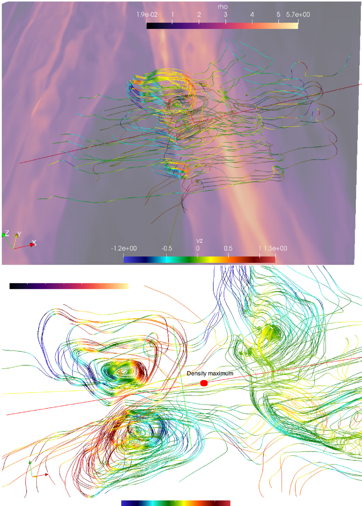
Figure 9. Streamlines associated with a spiral wave in a shearing box simulation of GI. The top panel is a view from the top (looking down to the mid-plane) while the bottom panel is a poloidal cut (view from the disc mid-plane) with the angular momentum vector pointing upward. The red line in the bottom panel indicates the mid-plane z = 0 . The colour of the streamlines represents in both cases the amplitude of the velocity component v_z .
