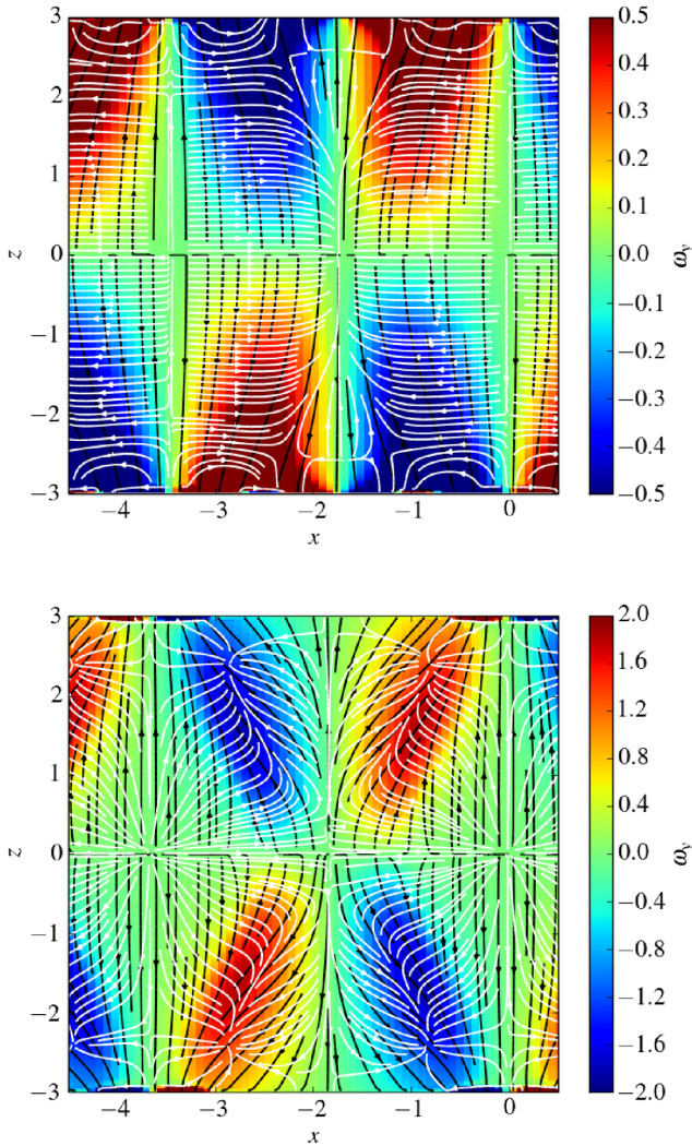
Figure 8. Vorticity in the y -direction for the case s = 20 and A = 0.05 (top) and A = 0.3 (bottom); the snapshot is zoomed in on one spiral arm of Fig. 6. The arrows represent the direction of the temperature (white) and entropy (black) gradients.
