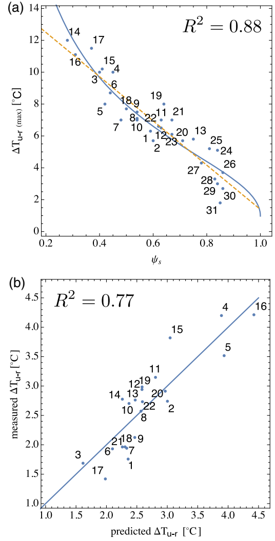
FIG. 4. Relationship between measured and model-predicted \Delta T_{u-r} . (a) Maximal \Delta T of group B cities as a function of the sky view factor \psi_s from Oke [33], together with the linear fit of Oke (dashed line) and the fit to our model (solid curve), from Eq. (2). Numbers in the figure correspond to cities analyzed by Oke [33]. (b) Comparison of measured and predicted \Delta T_{u-r} for group A cities using Eq. (1).
