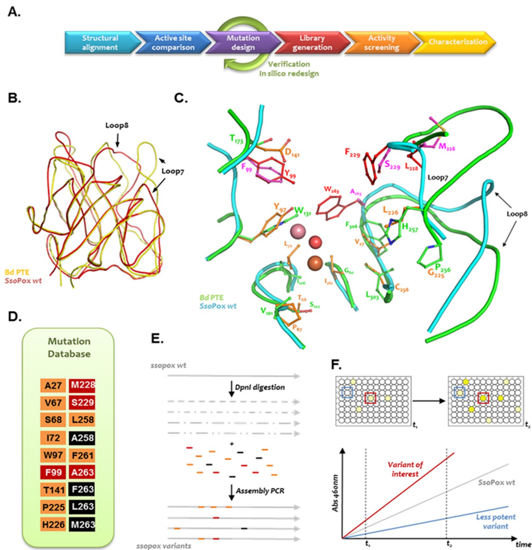
Figure 1. Structure-based design approach. (A) Pipeline used for the selection of improved mutants. (B) Structural alignments of SsoPox (red) and BdPTE structures (yellow) guided the mutational design. (C) Active site superposition of BdPTE (green) and SsoPox (cyan) active sites. Residues with structural equivalent (orange sticks) in both structures were used to design mutations of SsoPox 's residues into the BdPTE corresponding residues. Positions with no structural equivalent (red sticks) were designed using modelling tools (purple sticks) to mimic the active site cavity size, shape and chemical properties of the BdPTE crystal structure model (Figure S1). (D) The mutations data base consists of mutations to the BdPTE sequence when there is a structural equivalence (orange), and of mutations designed when there is no structural equivalence (red). The third set of mutations (black) adds more diversity at two selected positions, 258 and 263. (E) Once the library had been validated, primers carrying mutations were used to shuffle them and generate a gene library with random combinations of selected mutations. (F) The library was screened for paraoxonase activity to identify enzymes with improved proficiency.
