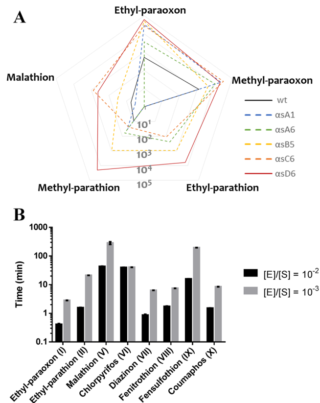
Figure 3. Activity characterization of the improved variants and bioremediation potential. (A) Phosphotriesterase catalytic efficiency comparison between wt- SsoPox and the best selected variants. Data for wt- SsoPox are from Hiblot et al. 46 . (B) Determination of the reaction time for hydrolyzing 95% using the \alpha sD6 variant of a solution of pesticide at 250 \mu M. Two enzyme-to-substrate ratios ( [E]/[S] ), 10^{-2} and 10^{-3} , were considered.
