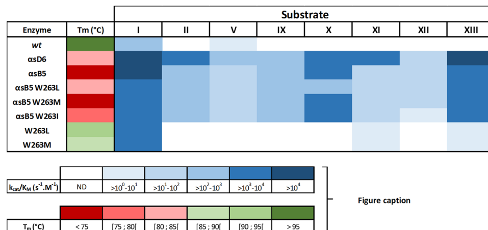
Figure 7. Overview of SsoPox wild-type and variants properties. Catalytic efficiencies towards organophosphate-based pesticides are presented using a color code ranging from white to dark blue. Melting temperatures are presented using a color code ranging from red to green.
