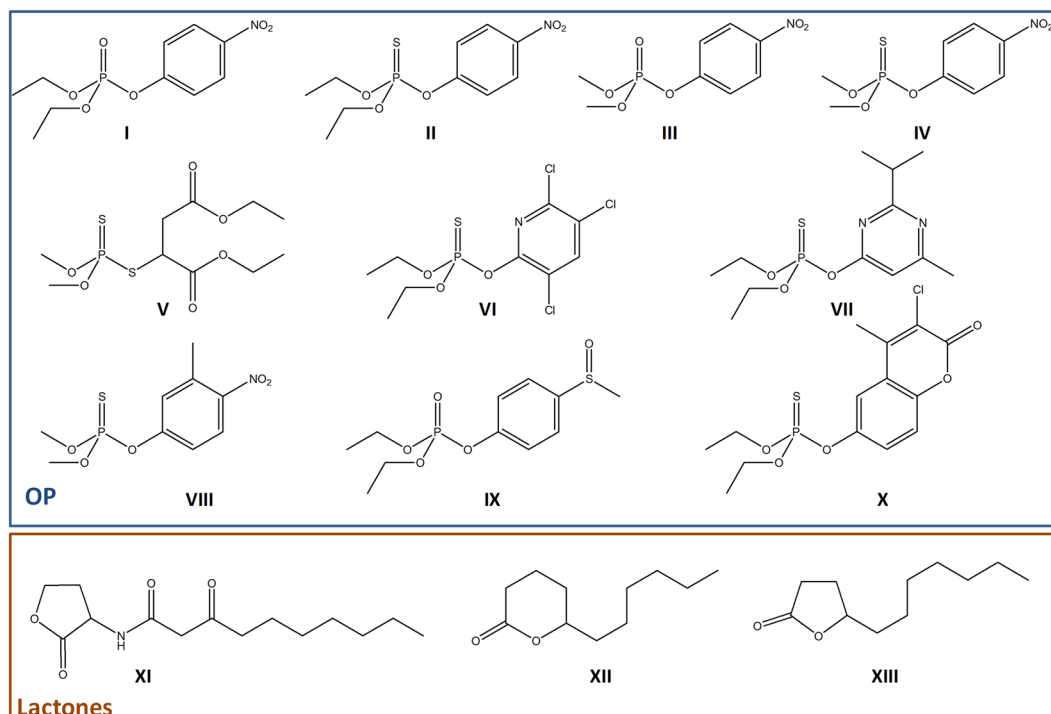
Figure 2. Chemical structure of substrates used in this study. The chemical structure of ethyl-paraoxon (I), ethyl-parathion (II), methyl-paraoxon (III), methyl-parathion (IV), malathion (V), chlorpyrifos (VI), diazinon (VII), fenitrothion (VIII), fensulfothion (IX), coumaphos (X), 3-oxo-C10 AHL (I) (XI), undecanoic- \gamma -lactone (XII) and undecanoic- \delta -lactone (XIII) generated using ChemDraw software.
