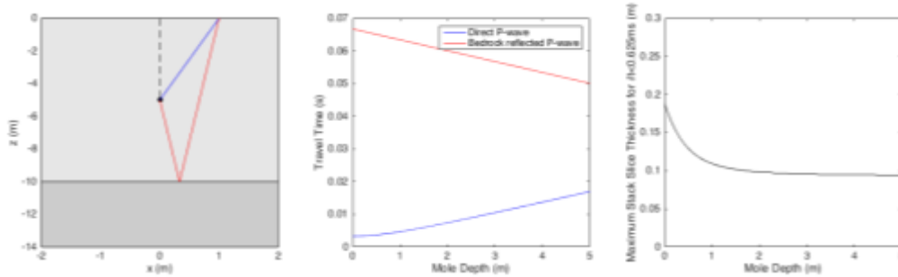
Figure 14: Stack depth slice requirements for a uniform regolith layer with a P-wave velocity of 300 m/s and a depth to bedrock of 10 m. (a) Sketch of ray paths for direct and reflected P-wave. (b) Travel time curves. (c) Maximum depth slice thickness over which traces can be stacked to ensure 1/16^{\text{th}} sample interval coherence of both reflected and direct phases.
