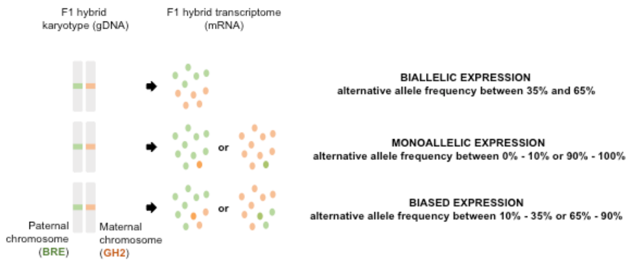
Figure 2: Detection Strategy of Parent-of-Origin Expression: example for Cross 1. Cross 1 was performed using males from the S. mansoni Brazilian strain (BRE), and females from the Guadeloupien strain (GH2). Each hybrid contains a chromosome from the mother (GH2) and from the father (BRE). The transcriptomic analysis of hybrid offspring allowed identifying genes i. expressed in equal proportions between the mother's (GH2) and father's (BRE) allele (i.e., biallelic expression), ii. expressed exclusively from the mother's (GH2) or father's (BRE) allele (i.e., monoallelic expression), or iii. expressed preferentially from the mother's (GH2) or the father's (BRE) allele (i.e., biased expression).
