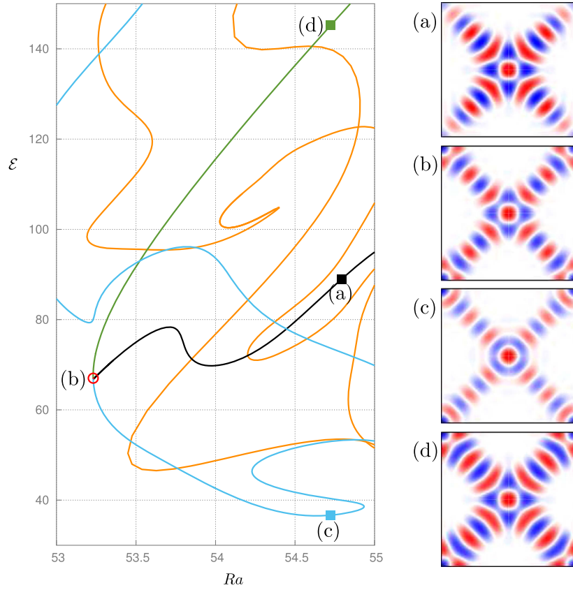
Figure 2. Spatial structures in the vicinity of the open red circle in figure 1, labeled (b), shown in terms of color-coded midlayer vertical velocity (blue: w(x, y, 1/2) < 0 , red: w(x, y, 1/2) > 0 ). The state (b) interpolates between three distinct state types, labeled (a), (c) and (d). We refer to states of this type as extended, to distinguish them from both localized states and domain-filling states. Domain size: 6\lambda_c \times 6\lambda_c \times 1 .
