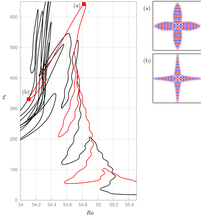
Figure 14. Left panel: detail of the bifurcation diagram in figure 11, with the black curve representing D_4 -symmetric states and the red curve D_2 -symmetric states. Right panels: four-armed D_2 -symmetric states at locations (a) Ra \approx 54.82 , (b) Ra \approx 54.11 shown in the left panel, both shown in terms of color-coded midlayer vertical velocity (blue: w(x, y, 1/2) < 0 , red: w(x, y, 1/2) > 0 ). Domain size: 18\lambda_c \times 18\lambda_c \times 1 .
