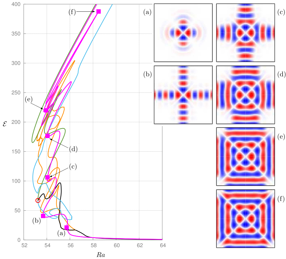
Figure 7. Spatial structure of D_2 -symmetric states with four arms oriented along the principal axes at several different locations along the (pink) solution branch. The first five of these locations correspond to the first five left folds ((a) Ra \approx 55.73 , (b) Ra \approx 53.69 , (c) Ra \approx 54.05 , (d) Ra \approx 54.07 , (e) Ra \approx 53.96 ); the last panel (f) shows an almost domain-filling state at Ra \approx 58.48 . The solution profiles are shown in terms of color-coded midlayer vertical velocity (blue: w(x, y, 1/2) < 0 , red: w(x, y, 1/2) > 0 ). The branches of D_4 -symmetric states from figure 1 are included in the left panel for comparison. Domain size: 6\lambda_c \times 6\lambda_c \times 1 .
