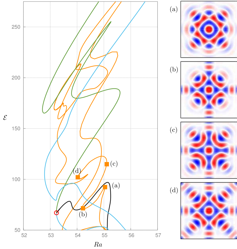
Figure 6. Continuation of figure 5 showing the evolution of the solutions along the pseudo-isola (orange curve). Spatial structure of an 8-fold state at (a) a right fold at Ra \approx 55.05 , (b) the next left fold at Ra \approx 54.22 , (c) the next right fold at Ra \approx 55.10 and (d) the next left fold at Ra \approx 54.03 , showing the growth of an eight-armed structure as one proceeds upwards along the orange branch. The solution profiles are shown in terms of color-coded midlayer vertical velocity (blue: w(x, y, 1/2) < 0 , red: w(x, y, 1/2) > 0 ). Domain size: 6\lambda_c \times 6\lambda_c \times 1 .
