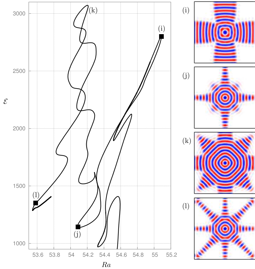
Figure 10. Left panel: detail of the bifurcation diagram in figure 9. Right panels: cross-like structures at locations (i) Ra \approx 55.087 , (j) Ra \approx 54.088 , showing the transition from cross-like growth to star-like growth, and fully developed starfish structures at locations (k) Ra \approx 54.189 , (l) Ra \approx 53.582 , all indicated in the left panel. The branch has been terminated at an arbitrary location near Ra \approx 53.8 . Domain size: 12\lambda_c \times 12\lambda_c \times 1 .
