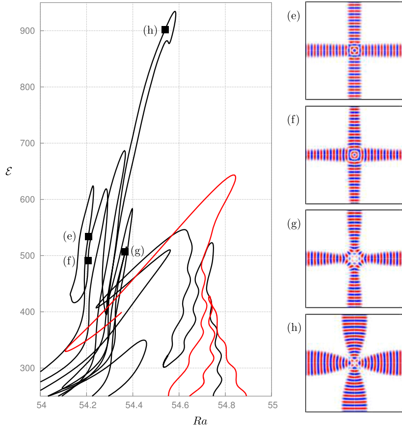
Figure 13. Left panel: detail of the bifurcation diagram in figure 11, with the black curve representing D_4 -symmetric states and the red curve D_2 -symmetric states. Right panels: four-armed D_4 -symmetric state at locations (e) Ra \approx 54.207 , (f) Ra \approx 54.206 , (g) Ra \approx 54.366 and (h) Ra \approx 54.539 shown in the left panel, all shown in terms of color-coded midlayer vertical velocity (blue: w(x, y, 1/2) < 0 , red: w(x, y, 1/2) > 0 ). Domain size: 18\lambda_c \times 18\lambda_c \times 1 .
