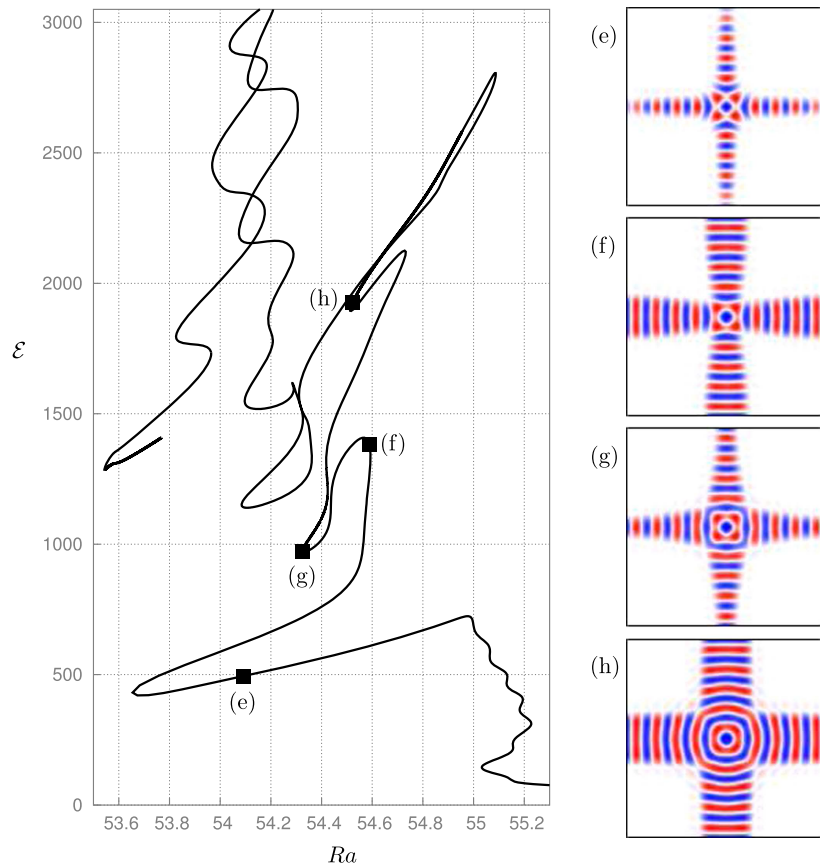
Figure 9. Left panel: continuation of the bifurcation diagram in figure 8. Right panels: cross-like structures at locations (e) Ra \approx 54.09 , (f) Ra \approx 54.59 , (g) Ra \approx 54.33 , (h) Ra \approx 54.52 indicated in the left panel, showing the growth of the ring structure around the core. The branch has been terminated at an arbitrary location near Ra \approx 53.8 . Domain size: 12\lambda_c \times 12\lambda_c \times 1 .
