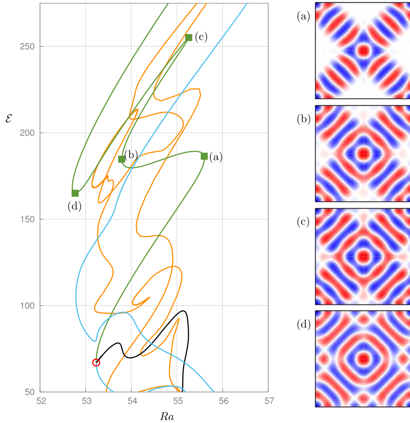
Figure 3. Spatial structure along the branch of spatially extended four-armed D_4 -symmetric states with arms along the diagonals (green curve) at (a) a right fold at Ra \approx 55.60 , (b) the next left fold at Ra \approx 53.79 , (c) the next right fold at Ra \approx 55.25 , and (d) the final left fold at Ra \approx 52.77 , showing the growth of the structure and its approach to a domain-filling convective state. The solution profiles are shown in terms of color-coded midlayer vertical velocity (blue: w(x, y, 1/2) < 0 , red: w(x, y, 1/2) > 0 ). A key state, indicated by an open red circle here and in figure 1, is shown separately in figure 2(b). Domain size: 6\lambda_c \times 6\lambda_c \times 1 .
