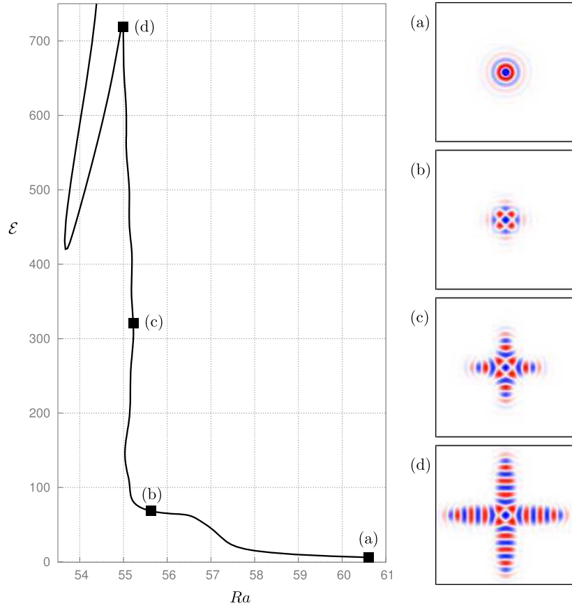
Figure 8. Left panel: bifurcation diagram showing the kinetic energy \mathcal{E} of D_4 -symmetric solutions as a function of the Rayleigh number Ra in a 12\lambda_c \times 12\lambda_c \times 1 domain. Right panels: a small amplitude target pattern at location (a) Ra \approx 60.60 and D_4 -symmetric localized states at location (b) Ra \approx 55.62 , (c) Ra \approx 55.22 and (d) Ra \approx 54.99 , all shown in terms of color-coded midlayer vertical velocity (blue: w(x, y, 1/2) < 0 , red: w(x, y, 1/2) > 0 ). The corresponding locations are indicated in the left panel. Domain size: 12\lambda_c \times 12\lambda_c \times 1 .
