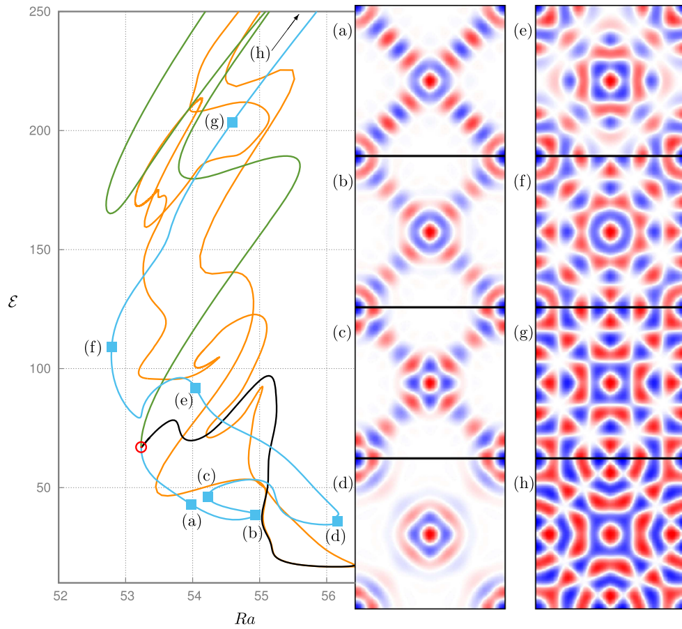
Figure 4. Spatial structure along the light blue branch of spatially extended four-armed D_4 -symmetric states below the open red circle in figure 1 showing a gradual transition from a four-armed state to a D_4 -symmetric domain-filling state via a spot-like pattern at location (d). The final state, shown at location (h), differs from the D_4 -symmetric domain-filling state in figure 3, location (d), obtained by following the green branch above the open red circle. The solution profiles are shown in terms of color-coded midlayer vertical velocity (blue: w(x, y, 1/2) < 0 , red: w(x, y, 1/2) > 0 ). Domain size: 6\lambda_c \times 6\lambda_c \times 1 .
