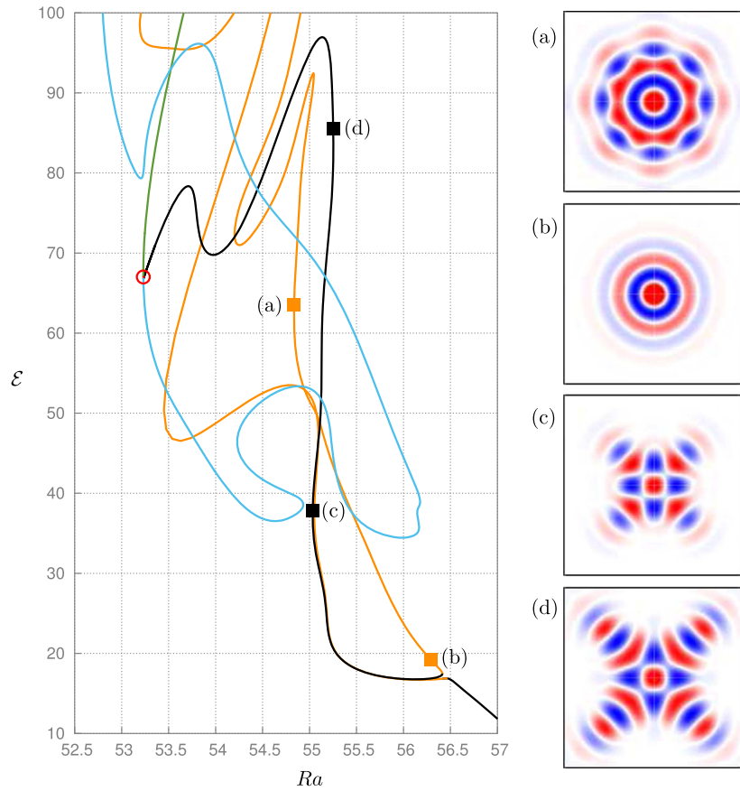
Figure 5. The transition from a four-armed structure with arms oriented along the diagonals (panel (c), Ra \approx 55.03 , and panel (d), Ra \approx 55.25 , black curve) to an eight-armed structure with arms oriented along both the diagonals and the principal axes of the domain (panel (a), Ra \approx 54.84 , orange curve) via a target pattern (panel (b), Ra \approx 56.29 ). The solution profiles are shown in terms of color-coded midlayer vertical velocity (blue: w(x, y, 1/2) < 0 , red: w(x, y, 1/2) > 0 ). Domain size: 6\lambda_c \times 6\lambda_c \times 1 .
