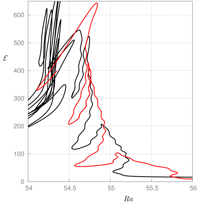
Figure 11. Bifurcation diagram for D_4 -symmetric states (black curve) and D_2 -symmetric states (red curve). The small oscillations in the center of the diagram correspond to nucleation of new rolls at the tips of the arms, while the large back-and-forth excursions are associated with the addition of a complete ring around the core. See Lo Jacono et al (2013) for details. This behavior terminates in prominent folds at the top center of the diagram, heralding the onset of interaction with image structures (top left of diagram). Domain size: 18\lambda_c \times 18\lambda_c \times 1 .
