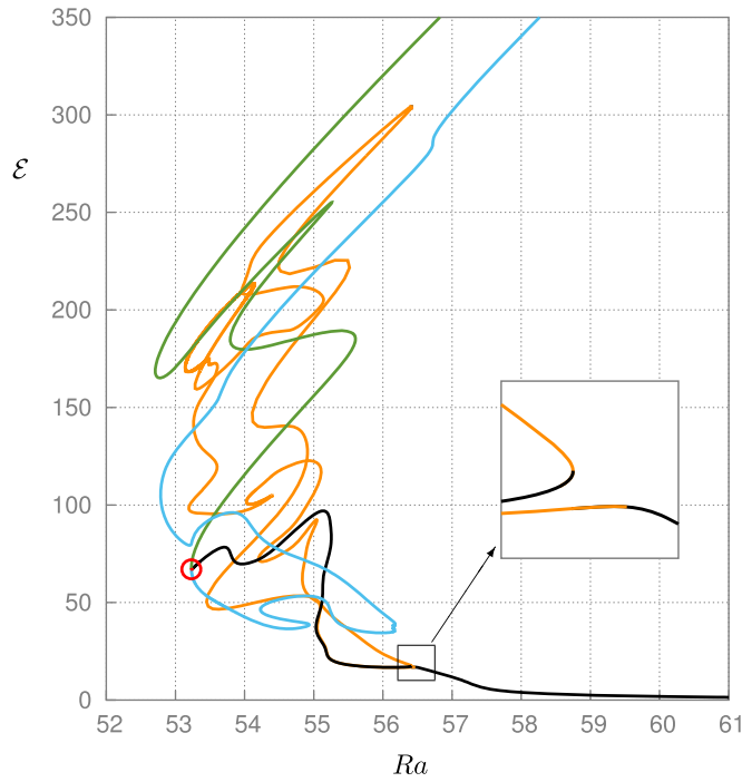
Figure 1. Bifurcation diagram for spatially extended D_4 -symmetric states with four arms along the diagonals (green curve) in a 6\lambda_c \times 6\lambda_c \times 1 domain showing the kinetic energy \mathcal{E} of the solution as a function of the Rayleigh number Ra . Superposed is a pseudo-isola of 8-fold states (orange curve) generated via an imperfect bifurcation (see inset) from a branch of localized D_4 -symmetric states (black curve) that originates at small amplitude near Ra_c \approx 66.657 (Lo Jacono et al 2013). These states peak in the center of the domain and differ from the states indicated in light blue which peak at the four corners. The open red circle indicates the bifurcation at which the two types of localized D_4 -symmetric structures (black and light blue curves) terminate on the branch spatially extended D_4 -symmetric states (green curve).
