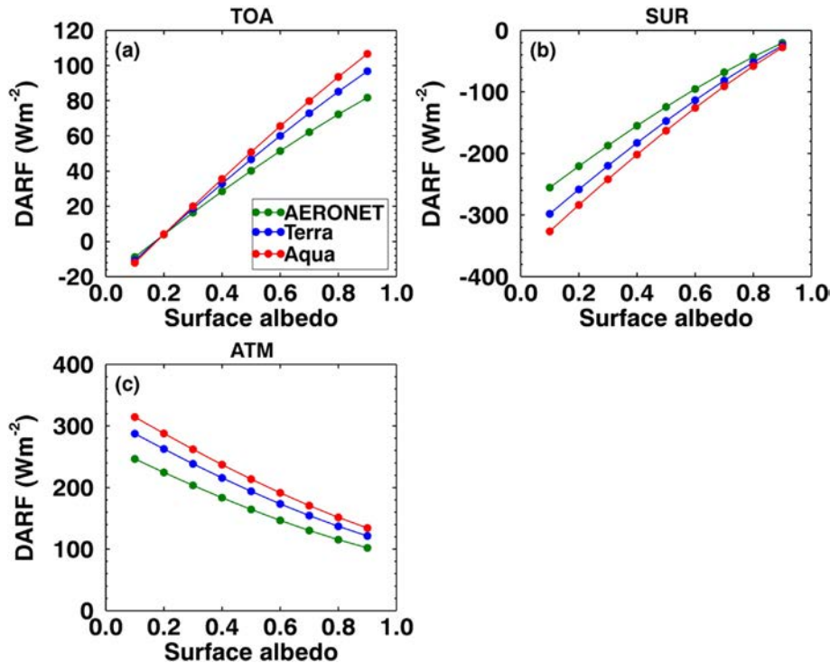
Fig. 9. Simulated daily averaged DARFs at TOA (a), at SUR (b), and in ATM (c) during the summertime based on the assumptions of various surface albedo, which take the following AODs as inputs into radiative transfer models: 1. hourly averaged AERONET-observed AOD in Fig. 3 (green solid circles); 2. constant MODIS/Terra AOD (blue solid circles); 3. constant MODIS/Aqua AOD (red solid circles). (For interpretation of the references to colour in this figure legend, the reader is referred to the web version of this article.)
