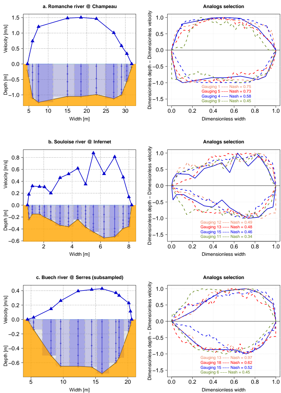
Figure 10: Illustration of the analogs selection for the three test cases. a. The Romanche river stream-gauging at Chapeau station (case 1). b. The Souloise river stream-gauging at Inernet station (case 2). c. Subsampled stream-gauging from Buech river at Serres station (case 3). For each case, scores printed on right hand graphs correspond to Nash values of the four best analogs. Gauging numbers refer to Table 1.
