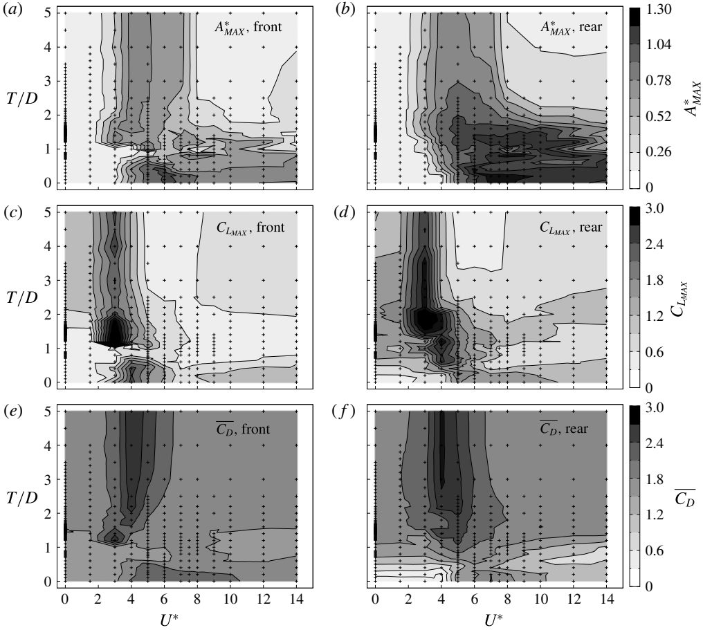
FIGURE 5. Over the U^*, T/D parameter space, (a,b) contours of maximum amplitude of oscillation, A_{MAX}^* , (c,d) contours of maximum coefficient of lift, C_{LMAX} , and (e,f) contours of mean coefficient of drag, \overline{C_D} . Maxima are calculated as an average of the greatest 10% of peaks. Panels on the left are for the upstream cylinder and on the right for the downstream.
