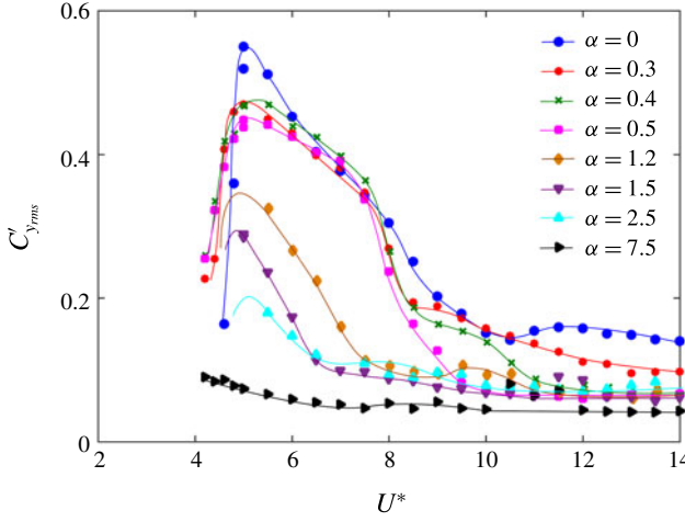
FIGURE 19. (Colour online) Variation of the C'_{y_{rms}} with reduced velocity for different rotation rates.
