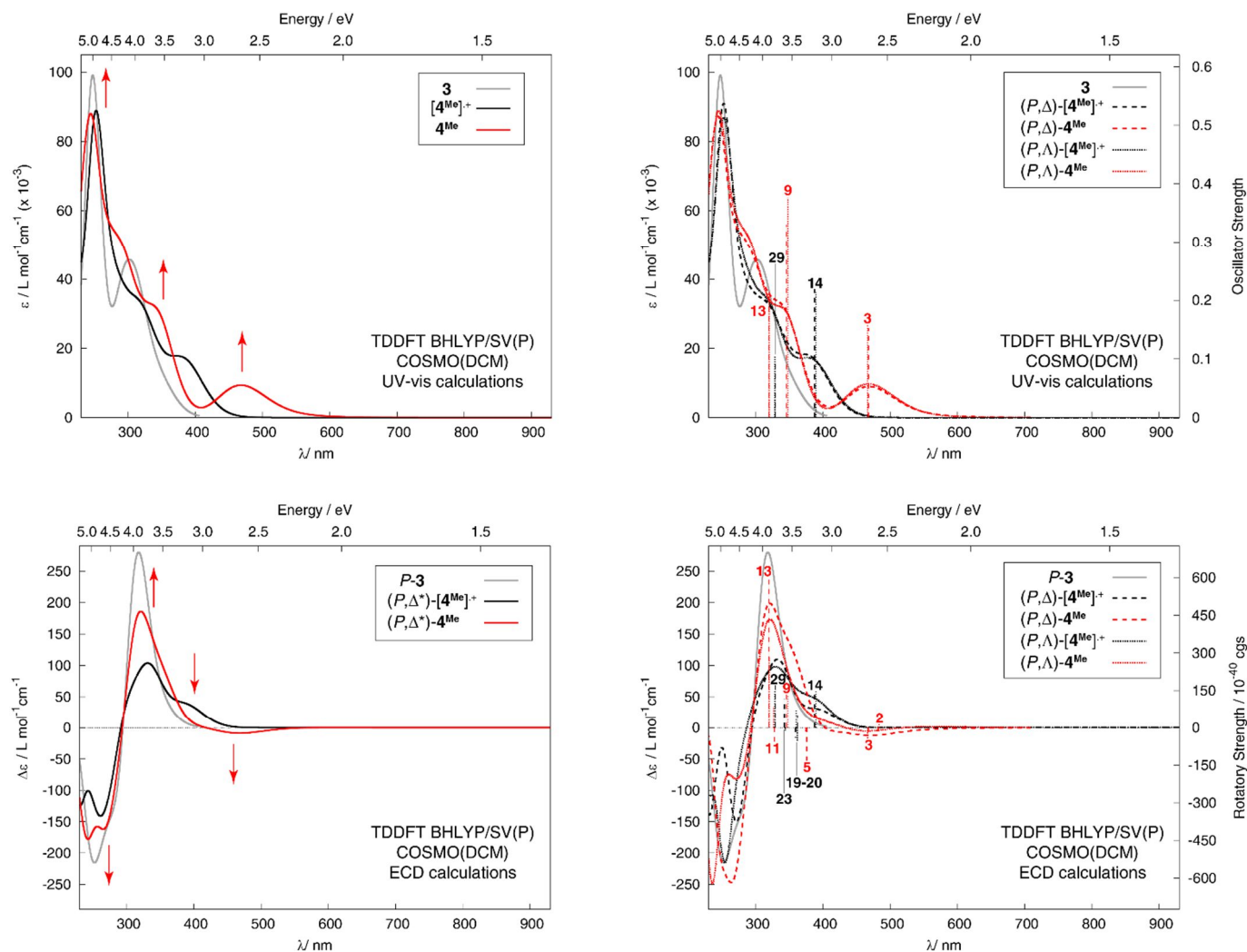
FIGURE 3. Comparison of the simulated (BHLYP) UV-vis (top) and ECD (bottom) spectra of (P,\Delta) -/ (P,\Lambda) - [4Me]^{+\bullet} , (P,\Delta) -/ (P,\Lambda) - 4Me^{\bullet} , their assumed 50:50 diastereomeric mixtures, (P,\Delta^*) - [4Me]^{+\bullet} and (P,\Delta^*) - 4Me^{\bullet} , and the bipyridine-[6]helicene 3 . No spectral shift has been applied. Calculated excitation energies and rotatory strengths indicated as ‘stick’ spectra. Numbered excitations correspond to those analyzed in detail (see also SI). Arrows indicate changes in the spectra due to the redox processes.
