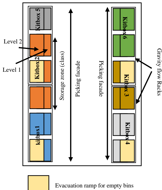
Figure 1: Top view of a detailed robotic kitting area layout
