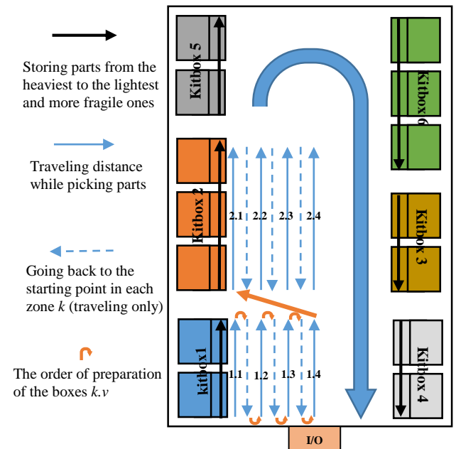
Figure 4: Representation the robot's traveling to prepare boxes k.v
