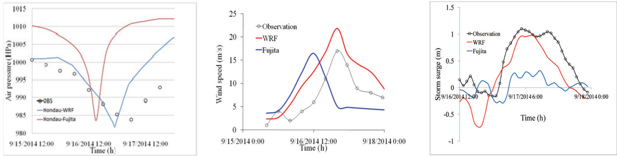
(a) Air pressure (b) Wind speed (c) Storm surges
