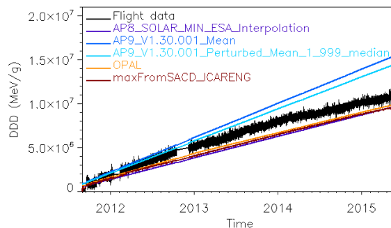
Fig. 6: Comparison of the measurements of the OSL DDD on board SAC-D spacecraft with those derived from the proton measurement with the ICARE-NG spectrometers, AP8 min, AP9 Mean V1.30.001, AP9 Perturbed Mean V1.30.001 median out of 40 scenarios and OPAL along a 660 km altitude, 98^\circ inclination orbit (after [8]).
