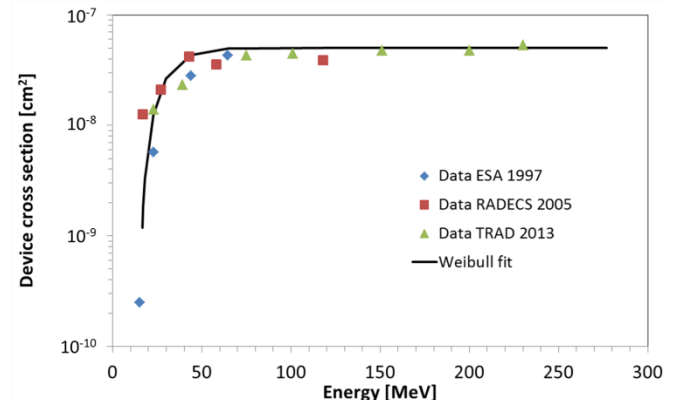
Fig. 10: M65608 SRAM device cross section versus proton energy.
