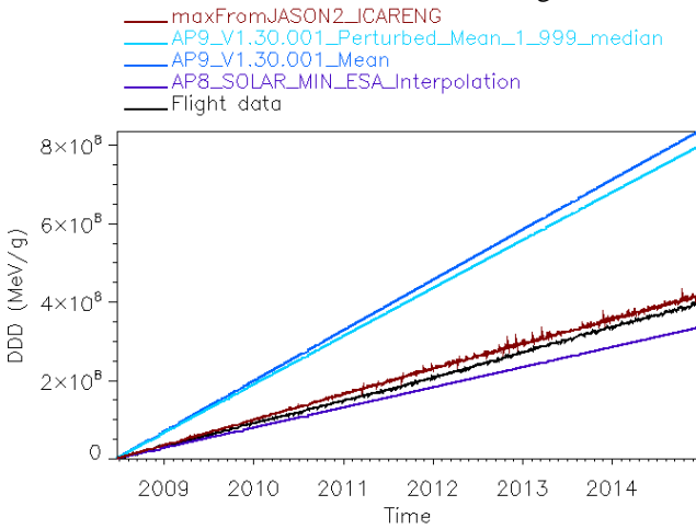
Fig. 15: Comparison of the measurements of the OSL DDD on board JASON-2 spacecraft with those derived from the proton measurement with the ICARE-NG spectrometers and AP8 min, AP9 Mean V1.30.001 and AP9 Perturbed Mean V1.30.001 median out of 40 scenarios along a 1336 km altitude, 63° inclination orbit (after [8]).
