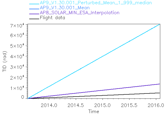
Fig. 21: Comparison of the measurements of the TID with those derived from AP8 min AP9 Mean V1.30.001 and AP9 Perturbed Mean V1.30.001 median out of 40 scenarios along a 8070 km altitude, 0° inclination orbit (after [8]). The two AP9 curves are overlapped.
