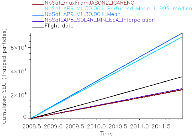
Fig. 18: Comparison of the cumulated SEUs measured by the EDAC on board JASON-2/SIRAL and predicted from AP8 min, AP9 V1.30.001 Mean and Perturbed mean-median out of 40 scenarios and OPAL models.
