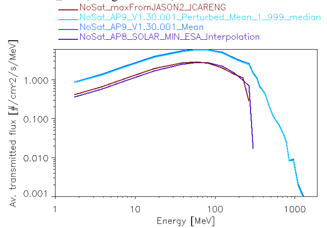
Fig. 17: Transmitted differential proton flux at the JASON-2/SIRAL/ chip level deduced from AP8 min and AP9 Mean V1.30.001, AP9 Perturbed Mean V1.30.001 median out of 40 scenarios models and JASON-2/ICARENG data.
