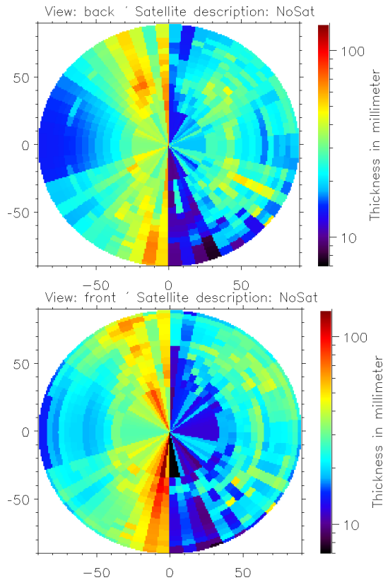
Fig. 9: "Fish eye" views of the shielding around the SRAM device on-board CRYOSAT-2 spacecraft; bottom is forward ( 2\pi steradians) and top is backward ( 2\pi other steradians). Color scale is in mm.
