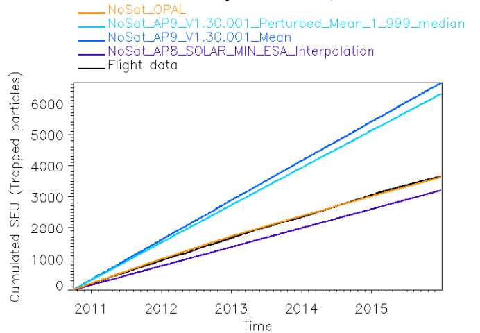
Fig. 14: Comparison of the cumulated SEUs measured by the EDAC on board CRYOSAT-2/SIRAL and predicted from AP8 min, AP9 Mean V1.30.001, AP9 Perturbed Mean V1.30.001 median out of 40 scenarios and OPAL models.
