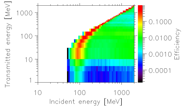
Fig. 13: Proton transport efficiency through the 3D shielding surrounding the chip on SIRAL payload.
