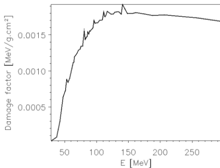
Fig. 4: Response function of damage factor of the OSL sensor on board SAC-D spacecraft considering isotropic proton incidence versus proton energy (after [8]).
