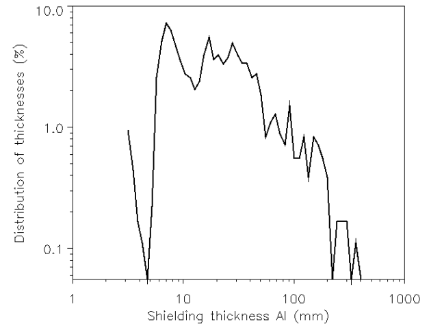
Fig. 2: Distribution of Al equivalent shielding thicknesses (in mm) as viewed by the OSL sensor on board SAC-D spacecraft (after [8]).
