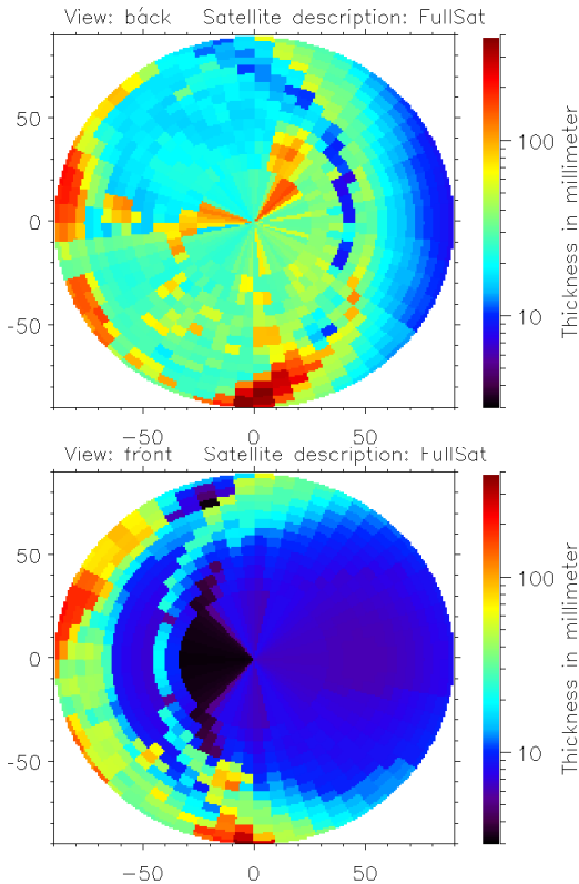
Fig. 3: "Fish eye" views of the shielding around the OSL sensor on-board SAC-D spacecraft; bottom is forward ( 2\pi steradians) and top is backward ( 2\pi other steradians). Color scale is in mm.
