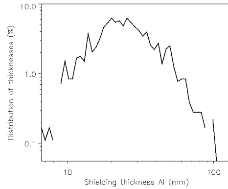
Fig. 8: Distribution of Al equivalent shielding thicknesses (in mm) as viewed by the SRAM device on board CRYOSAT-2/SIRAL spacecraft.
