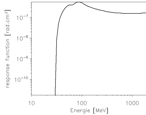
Fig. 20: Response function of ionizing dose factor of the RadFET implemented in the O3B/PLIU considering isotropic proton incidence versus proton energy (after [8]).
