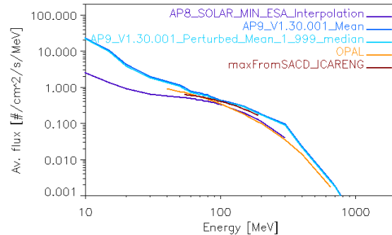
Fig. 5: Comparison of the mission average trapped proton spectrum at SAC-D orbit deduced from AP8 min, AP9 Mean V1.30.001, AP9 Perturbed Mean V1.30.001 median out of 40 scenarios, OPAL and ICARE-NG models and data.
