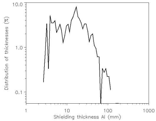
Fig. 19: Distribution of Al equivalent shielding thicknesses (in mm) as viewed by the RadFET on board O3B spacecraft (after [8]).
