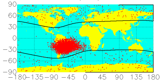
Fig. 7: SEU recorded by the EDAC implemented on the CRYOSAT-2/SIRAL payload from November 1 st , 2010 to December 31 st , 2015.
