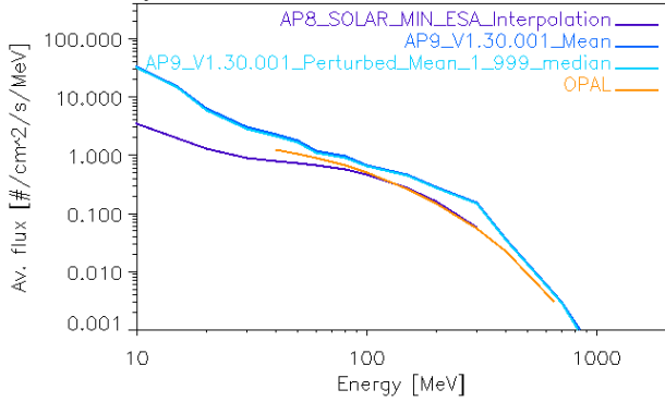
Fig. 11: Comparison of the mission average trapped proton spectrum at CRYOSAT-2 orbit deduced from AP8 min, AP9 Mean V1.30.001, AP9 Perturbed Mean V1.30.001 median out of 40 scenario and OPAL models.
