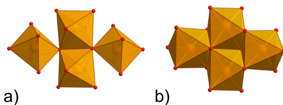
Fig. 1 Polyhedra representation of the butterfly topologies: a) {M 4 (μ 3 -O) 2 } and b) {M 4 (μ 3 -O) 2 (μ-O,N,X) 4 }.
