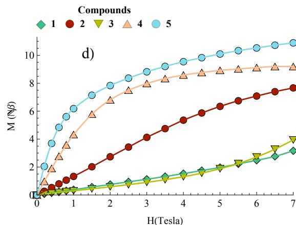
Fig. 4 a-c) Plots of c_M T vs. T measured from 300 to 2 K at 1 kOe for 1 (◆), 2 (●), 3 (▼), 4 (▲) and 5 (●), the solid black lines are the best-fit curves; d) plots of M vs. H measured from 0 to 7 T at 2 K for 1 (◆), 2 (●), 3 (▼), 4 (▲) and 5 (●), the solid lines are a guide for the eyes.
