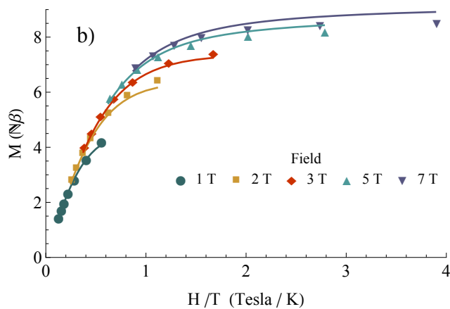
Fig. 5 a) M vs. H measured from 0 to 7 T and 1.8 K to 7.8 K for 4; b) Isofield M vs H/T from 1 T to 7 T for 4, the solid lines are the best-fit curves.
