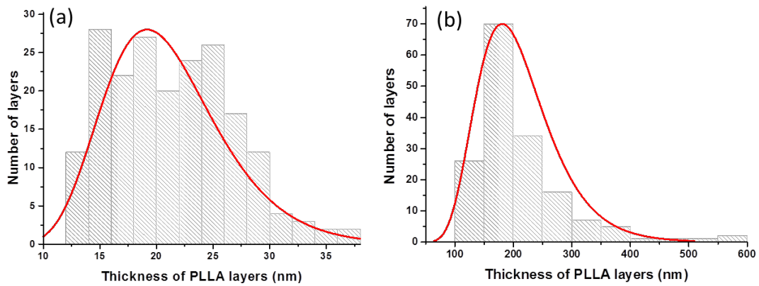
Figure 3. Distributions of PLLA layer thickness for the films containing 2049 layers (a) and 513 layers (b). The red lines represent the log-normal distribution curves.
