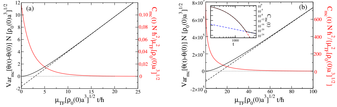
FIGURE 4: In the conditions of the figure 3, for a system prepared at t = 0 in the microcanonical ensemble at the temperature (a) k_B T = \mu_{\text{TF}} or (b) k_B T = 10\mu_{\text{TF}} , and isolated from its environment in its subsequent evolution, variance of the condensate phase shift \hat{\theta}(t) - \hat{\theta}(0) as a function of time t (solid line black) and its asymptotic diffusive behavior (80) (dashed). The correlation function C_{\text{mc}}(t) of d\hat{\theta}/dt is shown on the same figure in the secular-ergodic approximation (70) as a function of time (red solid line, ticks on the right) and, for (b), in an inset in log-log scale at long times (black solid line) to show that after a quasi-exponential decay in the root of time (fit with t^6 \exp(-C\sqrt{t}) in red dash) it follows a power law \propto t^{-5} (blue dashed). As in the figure 3, the multiplication of the quantities on the axes by well-chosen factors makes these results universal.
