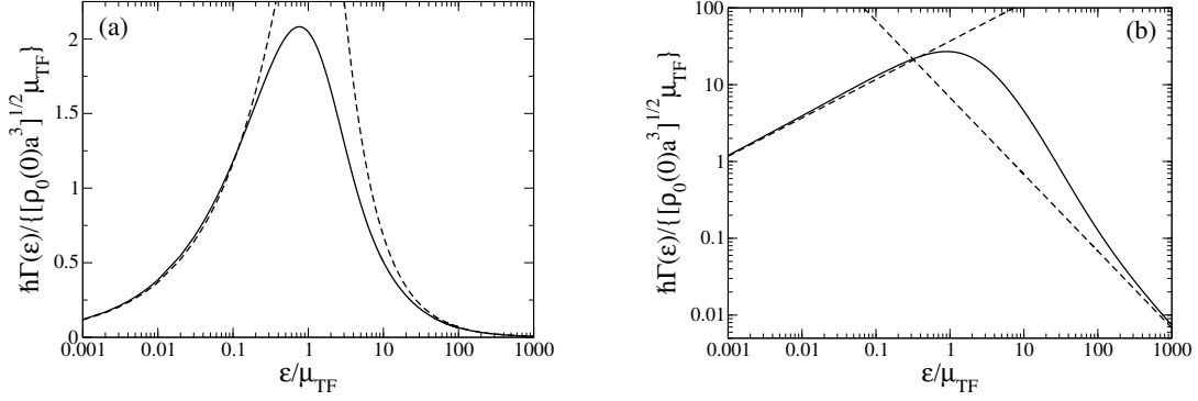
FIGURE 3: Beliaev-Landau damping rates \Gamma(\epsilon) of Bogoliubov modes of a condensate in a harmonic trap completely anisotropic as a function of the mode energy \epsilon , at the thermodynamic limit, in the secular-ergodic approximation (63, 64), at the temperature (a) k_B T = \mu_{\text{TF}} and (b) k_B T = 10\mu_{\text{TF}} , where \mu_{\text{TF}} is the Thomas-Fermi's chemical potential of the condensate. Thanks to the chosen units, the curve is universal; in particular, it does not depend on the trapping frequencies \omega_\alpha . The Bogoliubov modes considered must be in the classical motion regime \epsilon \gg \hbar\omega_\alpha and the system must be in the regime of an almost pure condensate, [\rho_0(\mathbf{0})a^3]^{1/2} \ll 1 and T \ll T_c , where \rho_0(\mathbf{0}) = \mu_{\text{TF}}/g is the density of the condensate in the center of the trap
