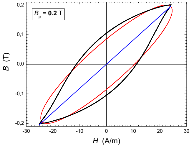
Fig. 2 – Experimental quasi-static loop at peak induction B_p = 0.2 T in the NO Fe-Si sheet. It is approximated either by a straight B(H) line ( \mu = 8.13 \cdot 10^{-3} Tm/A) or by the elliptic loop of identical area associated with the complex permeability \underline{\mu} = \mu' - j\mu'' , with \mu' = 7.35 \cdot 10^{-3} Tm/A and \mu'' = 3.47 \cdot 10^{-3} Tm/A.
