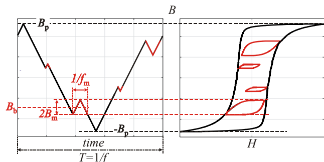
Fig. 1 – Example of PWM waveform and associated hysteresis cycles for a frequency modulation index of m_f = 5 . The major loop is in black; the nested minor loops are in red.
