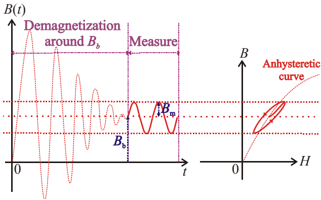
Fig. 4 – Acquisition method of the static complex permeability \underline{\mu}(B_m, B_b) on the an hysteretic curve as a function of peak and bias induction pair (B_m, B_b) . The bias value is generated by a third winding supplied by a stable constant current.
