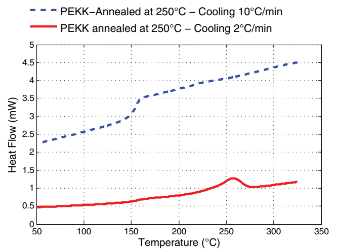
Fig. 7. DSC thermogram of PEKK: cooling ramps from melting state at 380^{\circ}\text{C} .
