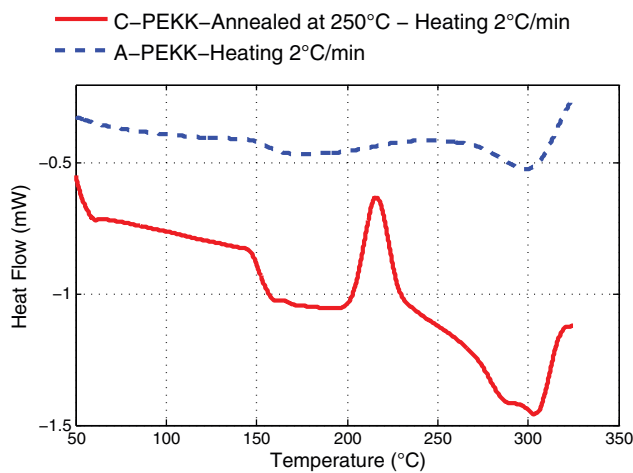
Fig. 6. DSC thermogram of A-PEKK and C-PEKK: first heating at 2^{\circ}\text{C}\cdot\text{min}^{-1} of molded samples.
