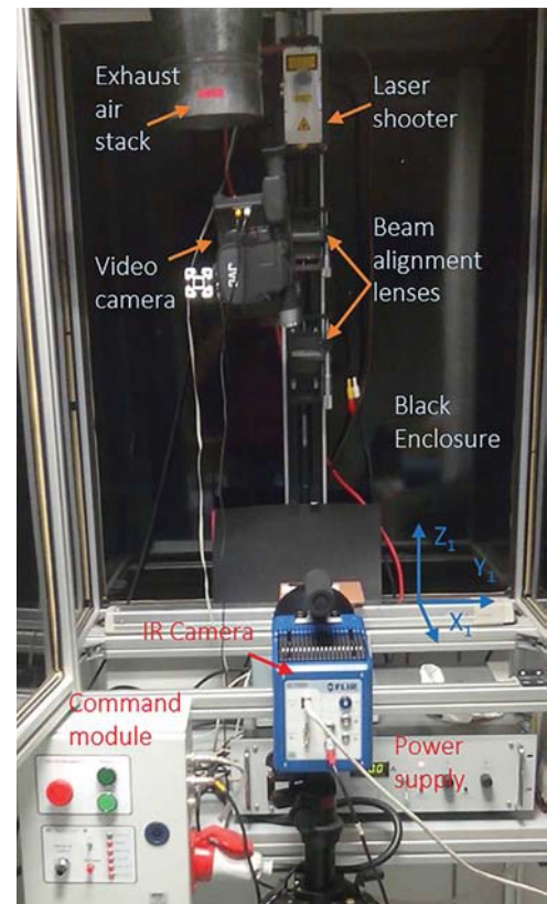
Fig. 4. Experimental laser device.
