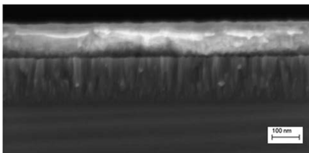
Figure 10. Left: Constant current charge-discharge cycles (1 st discharge cycle) of two gold electrodes. The measurement have been performed with and without the lithium diffusion barrier deposited in this study (TiN) in liquid electrolyte between 0.01 V and 1.5 V vs \text{Li}/\text{Li}^+ . Right: SEM cross section of the TiN/Au (2 nd sample) stacking sputtered on silicon substrate.
