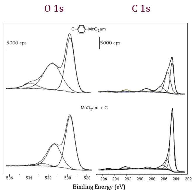
Figure 4. XPS O 1s and C 1s core level spectra of MnO 2 am- \phi -C and MnO 2 am + C.
