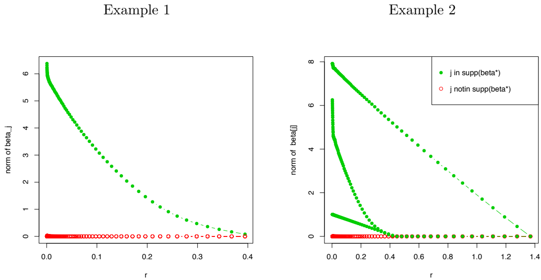
Figure 1: Plot of the norm of \left[\widehat{\beta}_{\lambda, \infty}\right]_j , for j = 1, \dots, 7 as a function of r .
