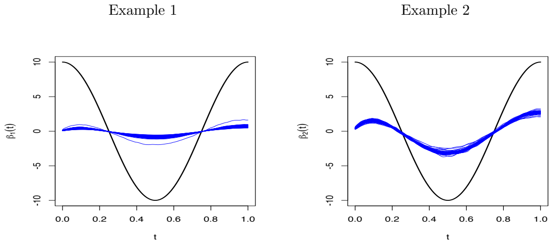
Figure 4: Plot of \beta_1^* (solid black line) and 50 Monte-Carlo replications of \left[\hat{\beta}_{\lambda, \hat{m}}\right]_1 (blue lines).
