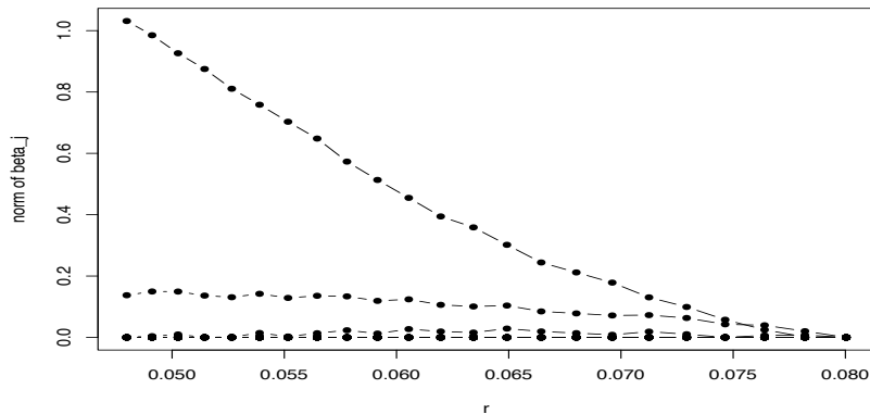
Figure 6: Plot of the norm of \left[\widehat{\beta}_{\lambda,\infty}\right]_j , for j = 1, \dots, 24 as a function of r .
