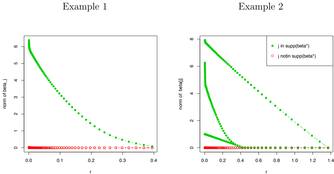
FIGURE 1. Plot of the norm of \hat{\beta}_j , for j = 1, \dots, 7 as a function of r .
