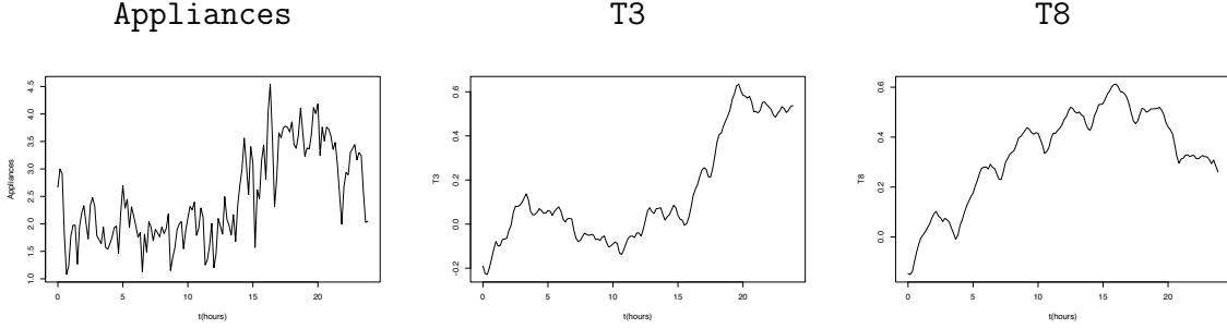
FIGURE 5. Plot of the \beta_j coefficients for j \in J(\hat{\boldsymbol{\beta}}) = \{1, 7, 17\} corresponding to the coefficients associated to the appliance energy consumption curve (Appliances), temperature of the laundry room (T3) and temperature of the teenage room (T8).
