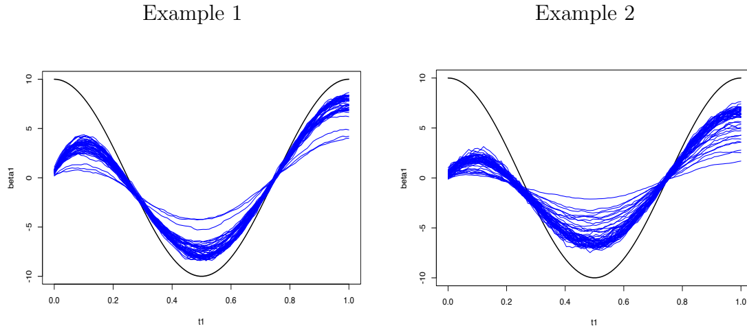
FIGURE 2. Plot of \beta_1^* (solid black line) and 50 Monte-Carlo replications of \hat{\beta}_1 (blue lines).
