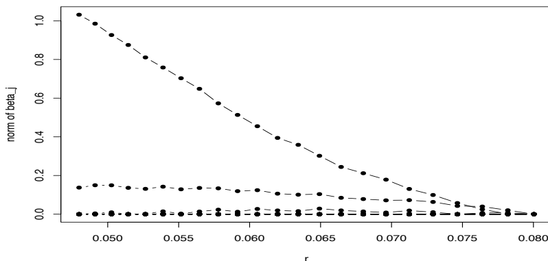
FIGURE 4. Plot of the norm of \widehat{\beta}_j , for j = 1, \dots, 24 as a function of r .
