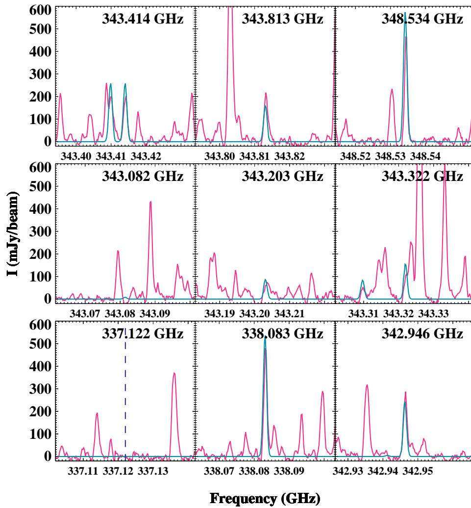
Figure B13. Nine selected lines of H 2 CS. Idem Fig. B1. The vertical blue dashed line in one of the panels indicates the position of the line that is too weak to generate an emission line under the assumed conditions.
