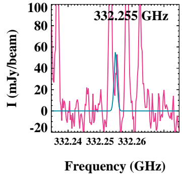
Figure B16. A selected line of HD 34 S. Idem Fig. B1.
