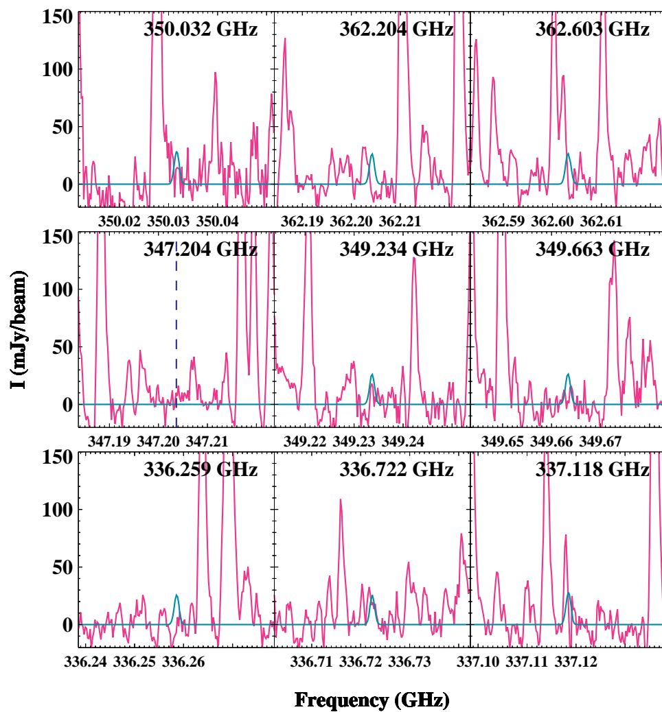
Figure B35. Nine selected lines of CCS. Idem Fig. B1. The vertical blue dashed line in one of the panels indicates the position of the line that is too weak to generate an emission line under the assumed conditions.
