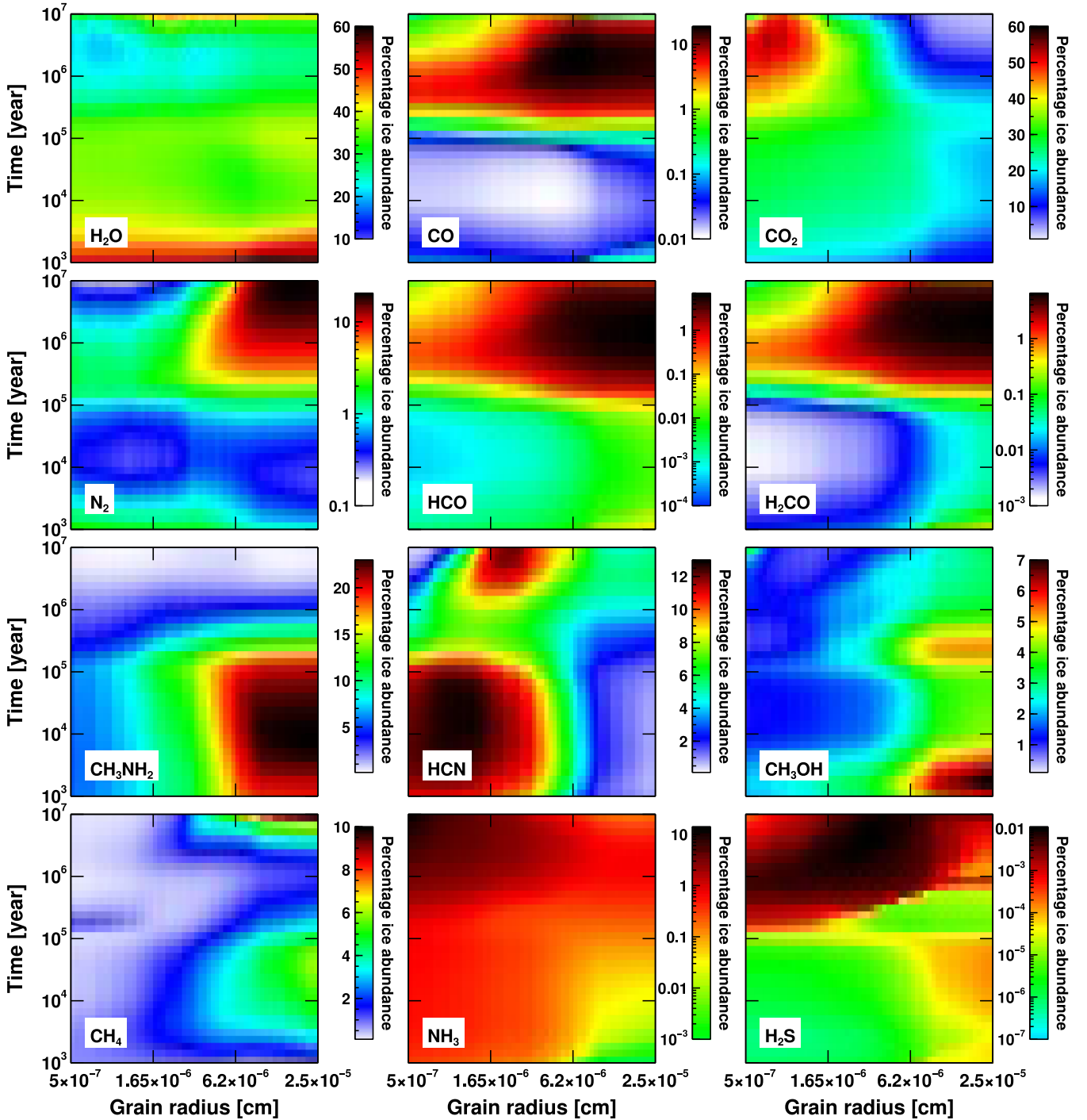
Fig. 16. Percentage ice abundances of the most abundant species as a function of grain size ( x -axis) and time ( y -axis). Results are for the multi grain model with 60 grain sizes and with non-uniform surface temperatures. The cosmic-ray-induced desorption is used and the MRN grain size distribution was used to calculate number density of 60 grain bins.
