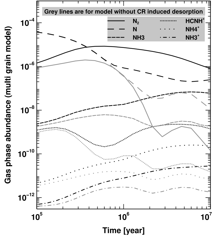
Fig. 10. Gas phase abundances of selected N-bearing species as a function of time as obtained in the multi-grain model with 60 bins and with the MRN grain size distribution. Black and grey lines are for the models with and without the cosmic-ray-induced desorption, respectively. The dust temperature is kept constant at 10 K in both models.
