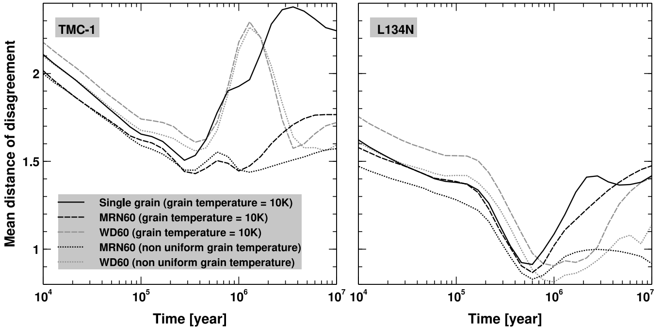
Fig. 19. Mean distance of disagreement computed for two dark clouds TMC-1 network and L134N.
