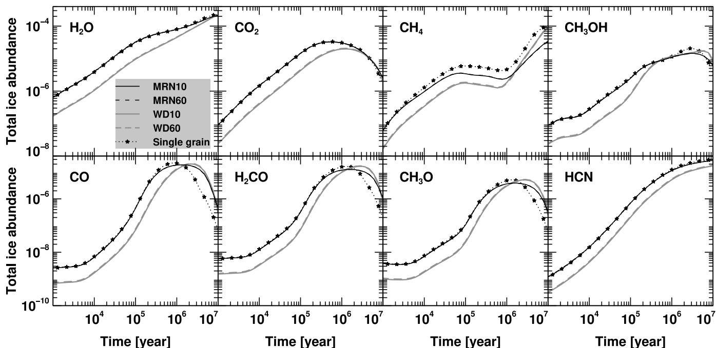
Fig. 13. The total ice abundances of selected species on dust grains as a function of time for models with different grain size distributions and a different number of bins. Legends apply to all panels.
