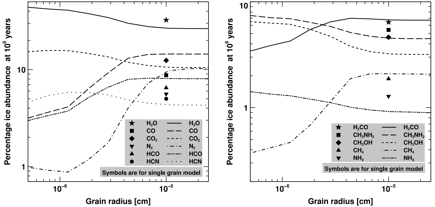
Fig. 7. Percentage ice abundances of the most abundant species as a function of grain radius at 10 6 yr. Results are for the simulation with the cosmic-ray-induced desorption enabled and for the multi-grain model (lines), with 60 grain sizes and the MRN grain size distribution, and the single-grain model (symbols). The dust temperature is kept constant at 10 K for all grains.
