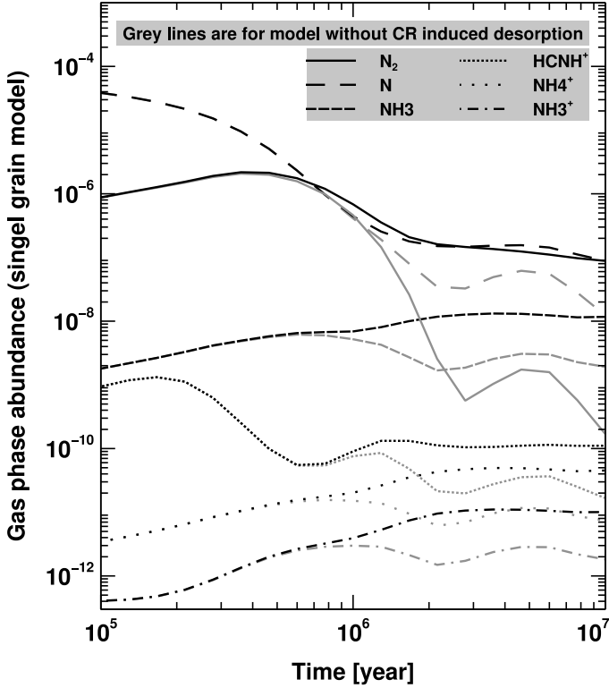
Fig. 9. Simulated results of gas phase abundances of selected N-bearing species as a function of time as obtained in the single-grain model. Black and gray lines are for models with and without cosmic-ray-induced desorption, respectively. Dust temperature is kept constant at 10 K in both models.
