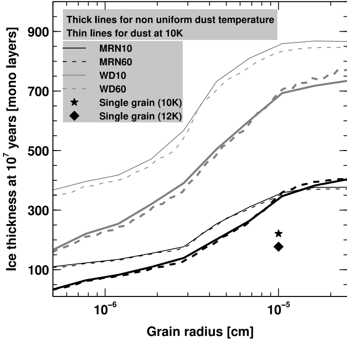
Fig. 15. The ice thickness as a function of grain radius at 10^7 yr in the different models. Thin lines: all grains have the same temperature of 10 K. Thick lines: all grains have their own temperature, see Fig. 3. Cosmic ray induced desorption is used in all models.
