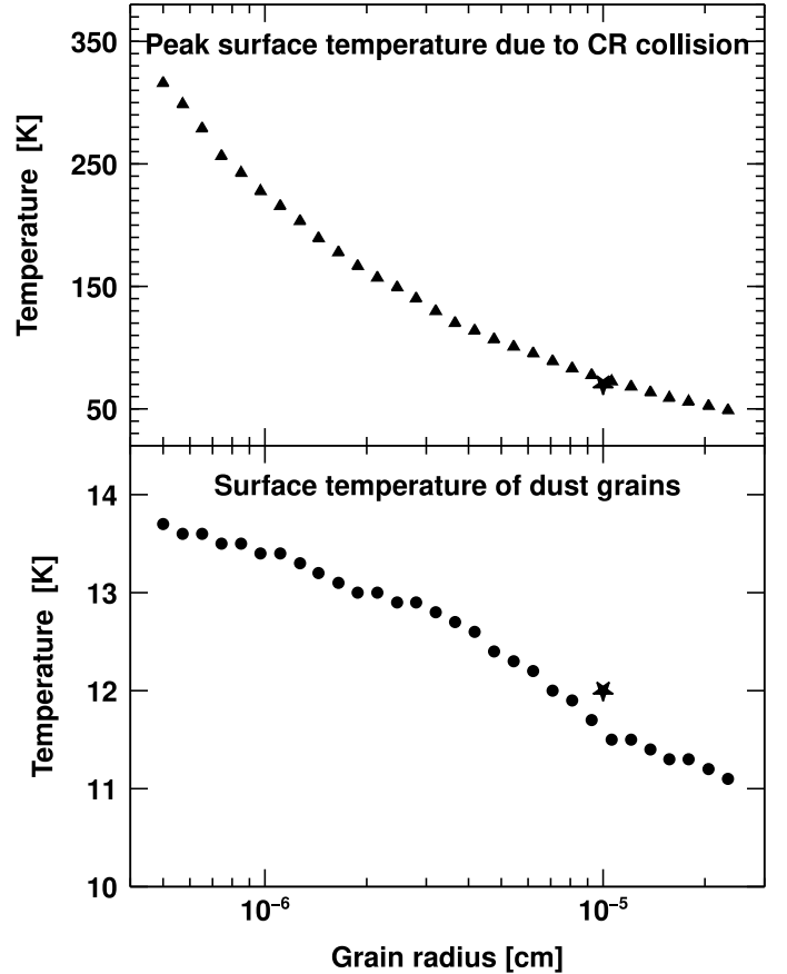
Fig. 3. Bottom panel: grain temperature (circles for multi-grain model and star for single-grain model) as a function of grain radius. Top panel: peak surface temperature (triangles for multi-grain model and star for single-grain model) due to collision with cosmic rays as a function of grain radius.
