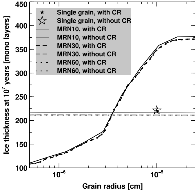
Fig. 4. Ice thickness as a function of grain radius for models with the MRN distribution and with the cosmic-ray-induced desorption enabled (black lines) and disabled (gray lines). Stars show the results for the single grain model. The dust temperature is kept constant at 10 K for all grains.
