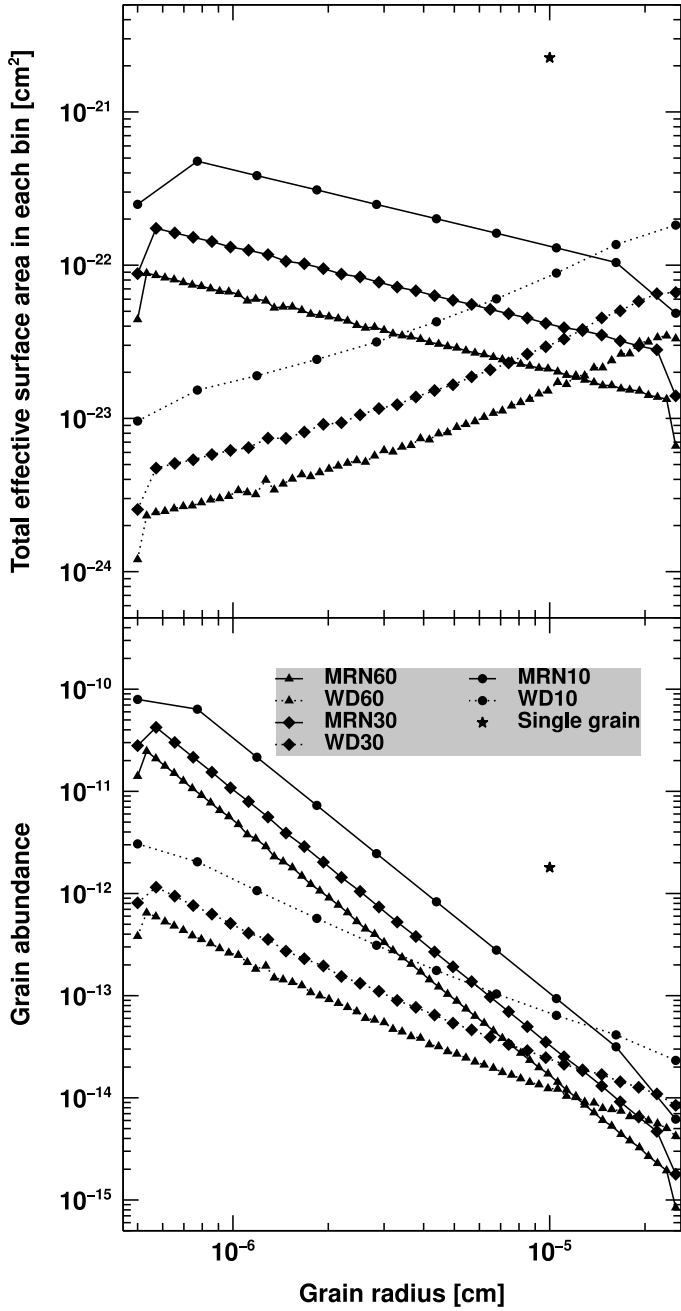
Fig. 2. Bottom panel: the grain abundance (with respect to the total proton density) in each bin plotted against the grain radius. Top panel: the total effective grain surface area (in \text{cm}^2 ) of each bin for different models plotted against the grain radius. Legends apply to both panels.
