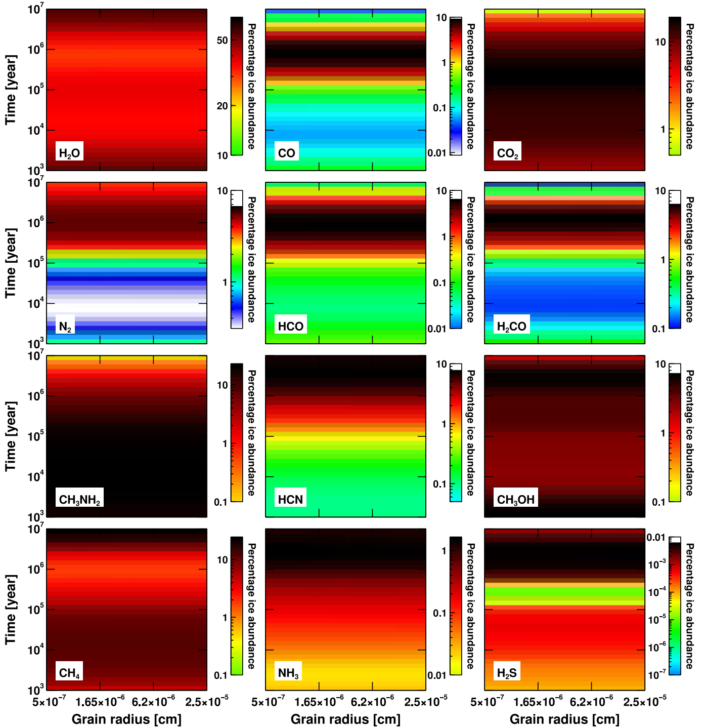
Fig. 6. As in Fig. 5 but without cosmic-ray-induced desorption.
