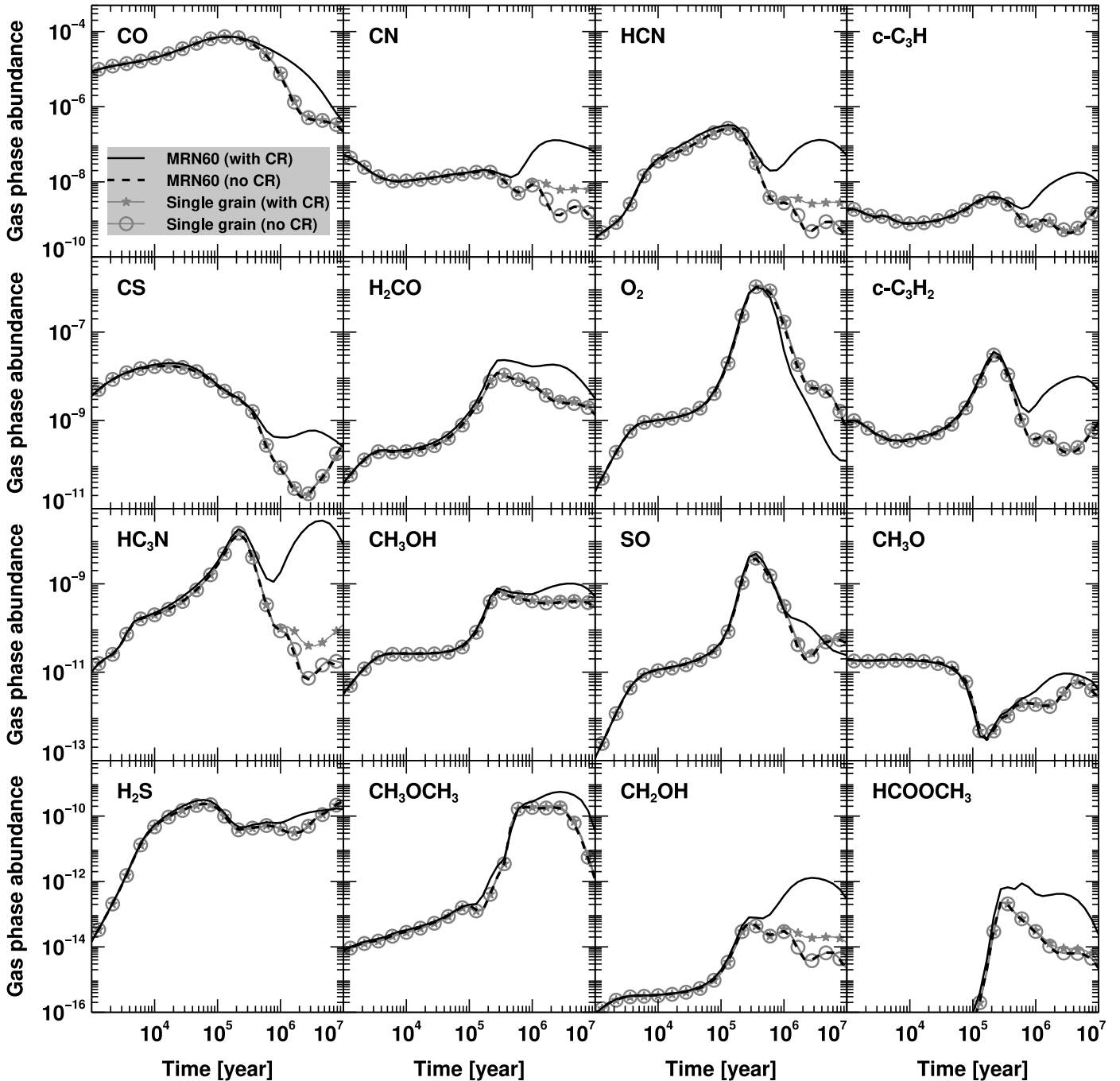
Fig. 8. Gas phase abundances of selected species as a function of time. Solid and dashed black lines are for the multi-grain models with the cosmic-ray-induced desorption enabled and disabled, respectively. Gray lines with stars and circles, respectively, show the results from the single-grain model with and without the cosmic-ray-induced desorption. The dust temperature in each model is kept constant at 10 K for all grains. Legends apply to all panels.
