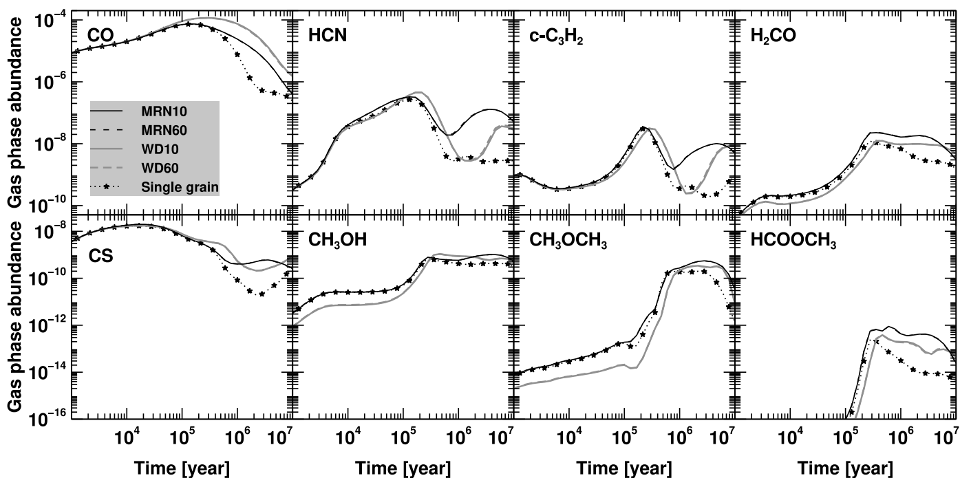
Fig. 14. Gas phase abundances of selected species as a function of time for models with different grain size distributions and a different number of bins. Legends apply to all panels.
