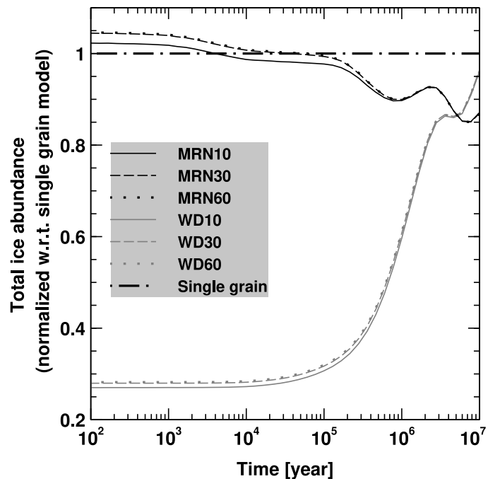
Fig. 11. Normalized total ice abundances as a function of time (see text). Cosmic-ray-induced desorption was enabled and the surface temperature was kept constant at 10 K in all models.
