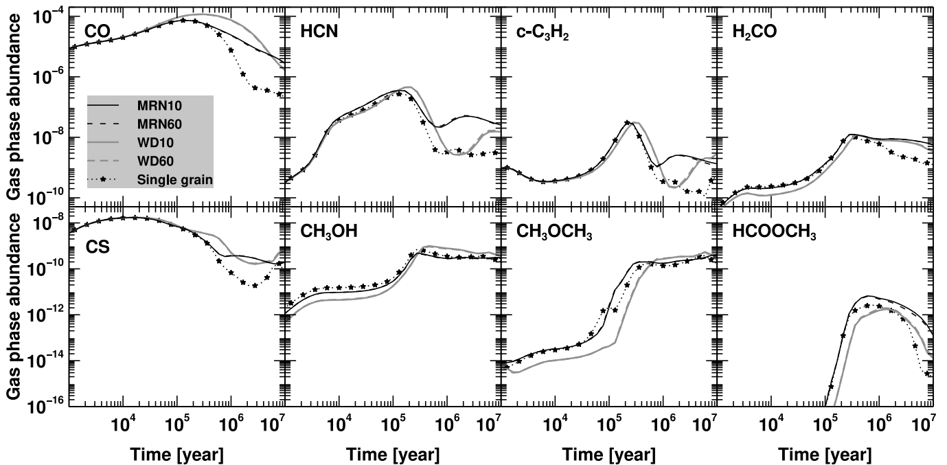
Fig. 18. Gas phase abundances of selected species as a function of time for models with different grain size distributions and a different number of bins. Grain temperature is nonuniform in the multi-grain models and in the single-grain model surface temperature is 12 K. This legend applies to all panels.
