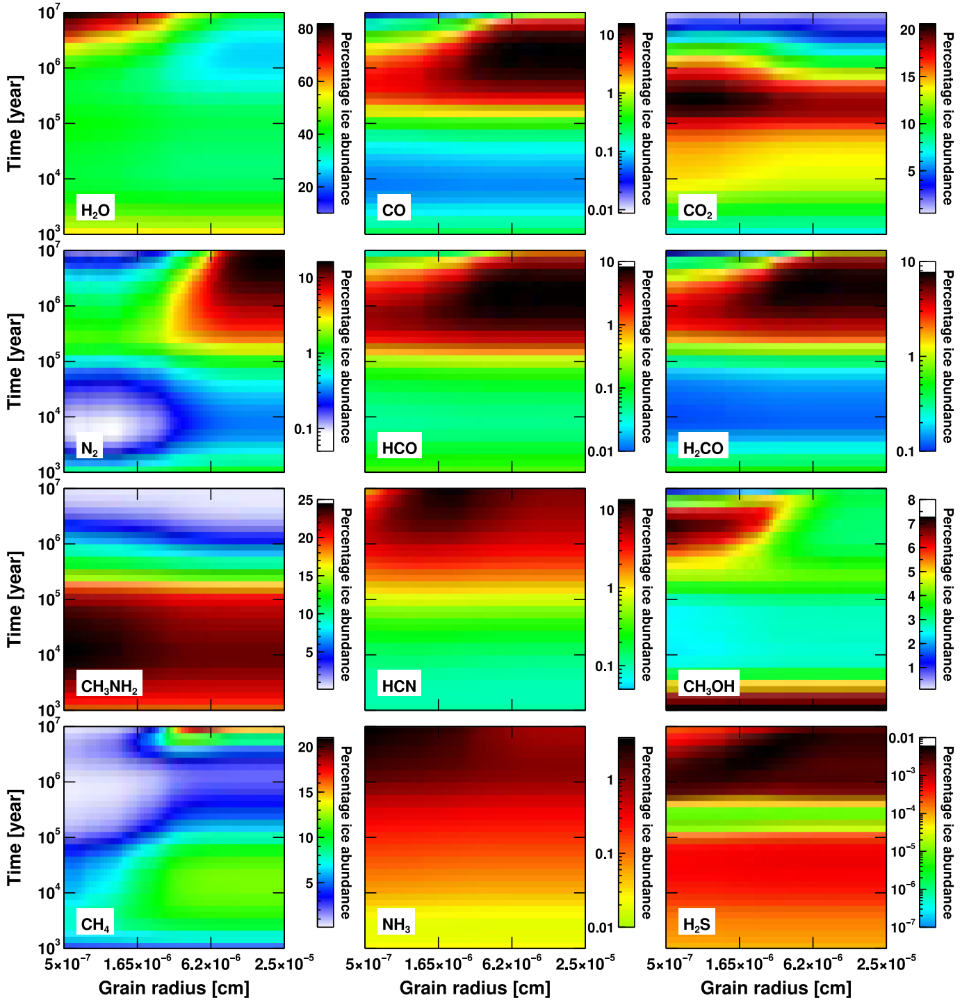
Fig. 5. Percentage ice abundance of the most abundant species as a function of grain radius ( x -axis) and time ( y -axis). Results are for simulation with cosmic-ray-induced desorption enabled and for the MRN grain size distribution with 60 grain sizes. The dust temperature is kept constant at 10 K for all grains.
