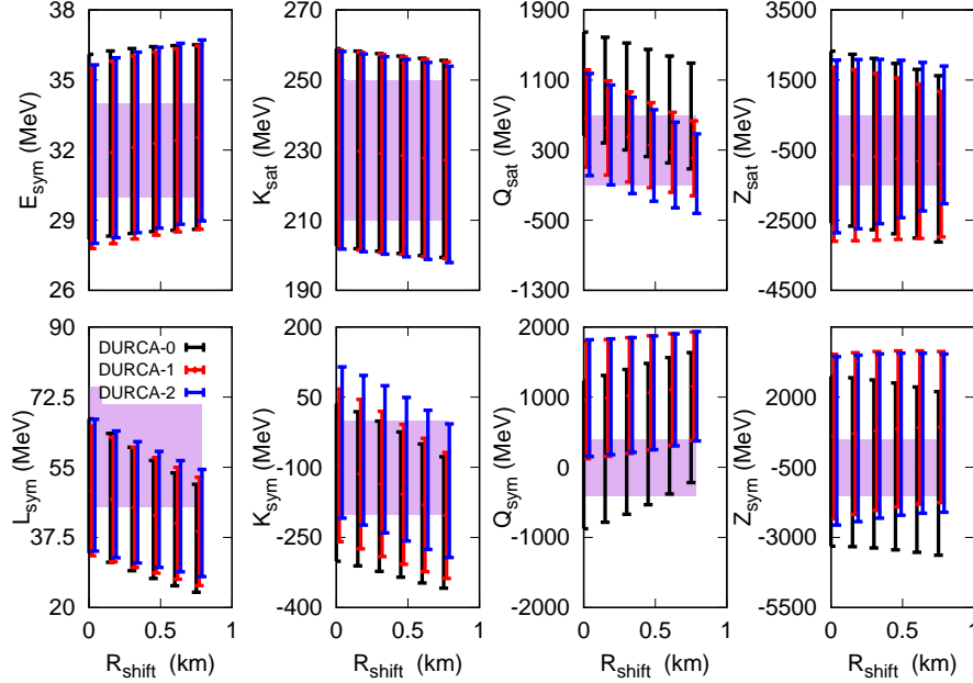
FIG. 21. (Color online) Effect of shifting the average radius by -R_{shift} on the empirical parameters. The purple 1-\sigma bands shown for each empirical parameter are deduced from Tab. I. See text for more details.
