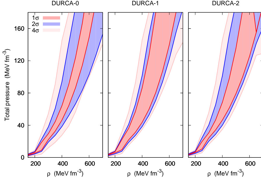
FIG. 18. (Color online) Total pressure function of the energy density \rho (including the rest mass contribution).
