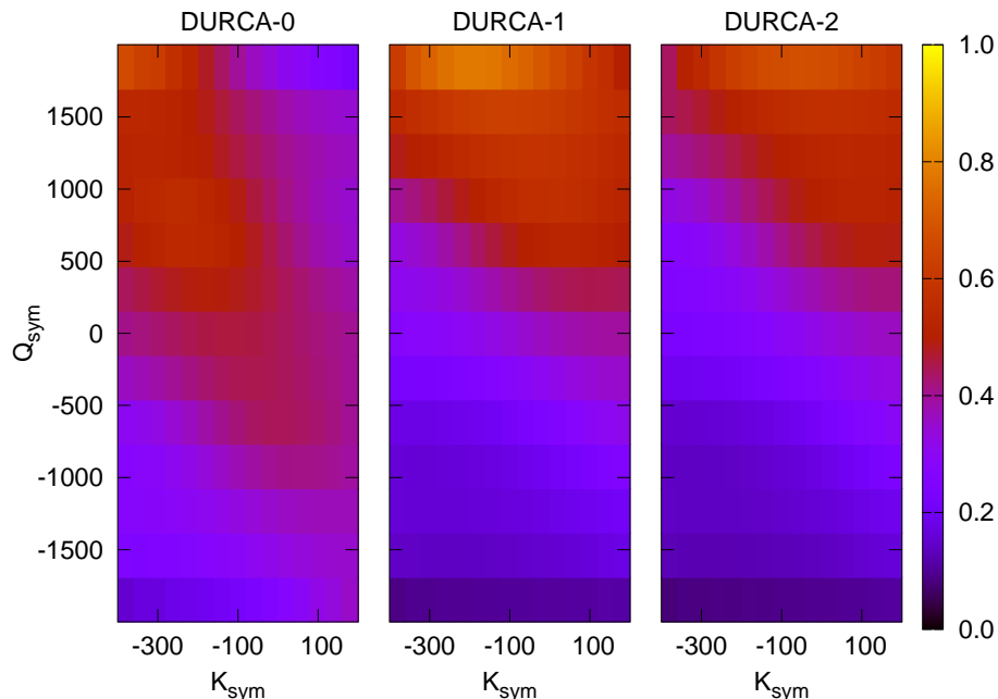
FIG. 6. (Color online) Two parameters probabilities showing the correlation between Q_{\text{sym}} and K_{\text{sym}} for DURCA-0, 1 and 2 (the prior is here taken uniform). The units on the axes are MeV.
