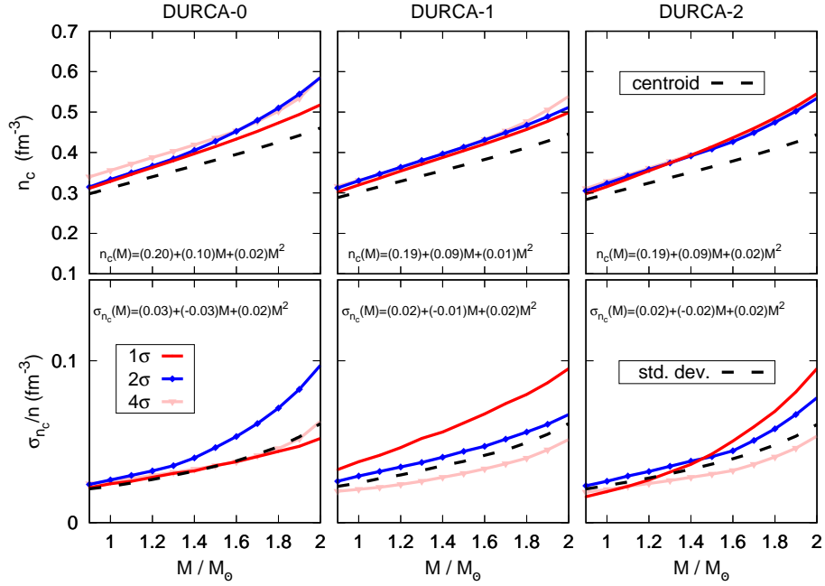
FIG. 13. (Color online) Same as Fig. 11 for the central density.
