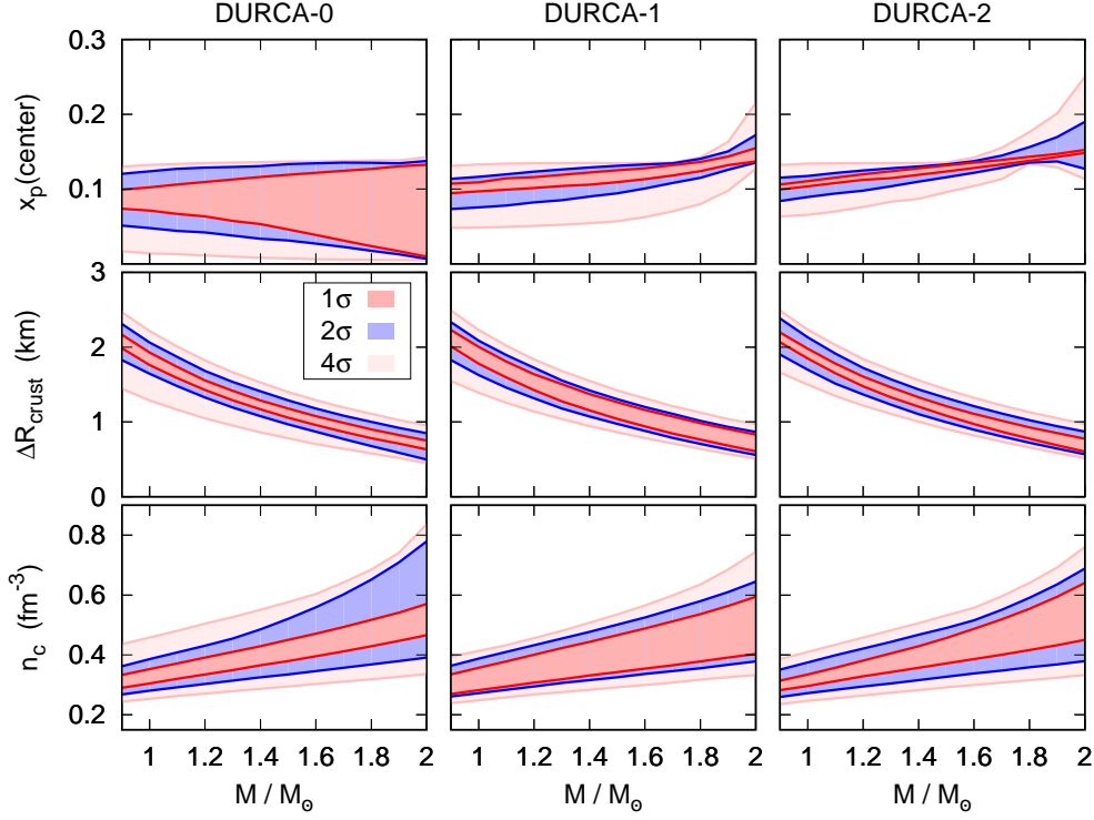
FIG. 9. (Color online) Same as Fig. 8 for the correlation between the central proton fraction x_p , crust thickness \Delta R_{crust} and central density n_c function of the mass.
