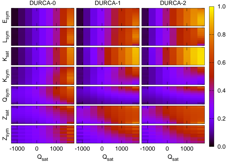
FIG. 5. (Color online) Two parameters probabilities function of Q_{sat} for DURCA-0, DURCA-1 and DURCA-2 (the prior is here taken flat). The units on the x-axis are MeV and the y-axes cover the range defined in Tab. I from bottom to top.
