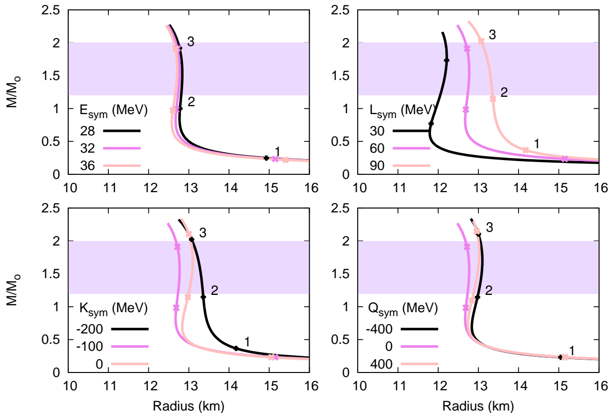
FIG. 3. (Color online) Same as Fig. 2 for the variation of isovector empirical parameters.
