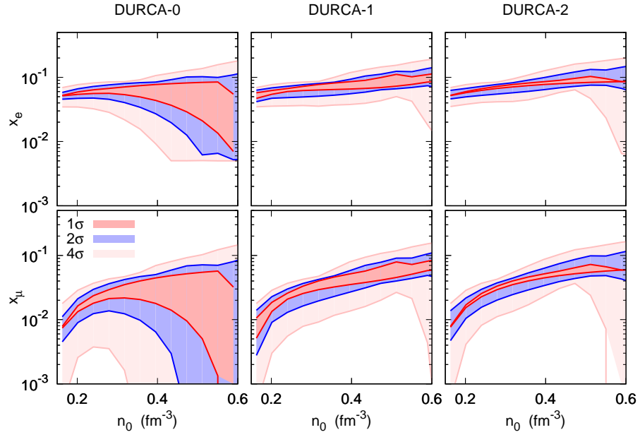
FIG. 16. (Color online) Same as Fig. 15 for the electron fraction x_e and muon fraction x_\mu .
