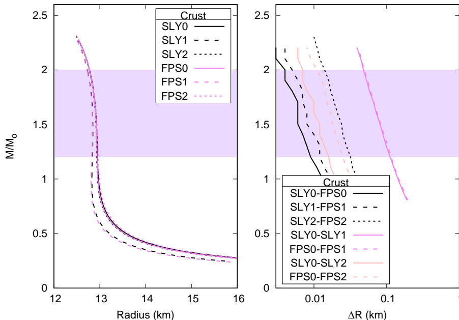
FIG. 1. (Color online) Effect of the crust and of the matching between the crust and the core EoS. Left part: mass-radius relationship with different prescriptions for the choice of the crust EoS and of the matching procedure (see text). Right part: sensitivity analysis of the shift in the NS radius induced by the different choices given in the legend of the figure (see text also). For instance, the solid black line stands for \Delta R = R(\text{SLY0}) - R(\text{FPS0}) . The largest impact is found for the modification of the low-density boundary of the matching between the crust and the core. Even for this extreme case, the uncertainty in the radius definition is less than 0.1 km.
