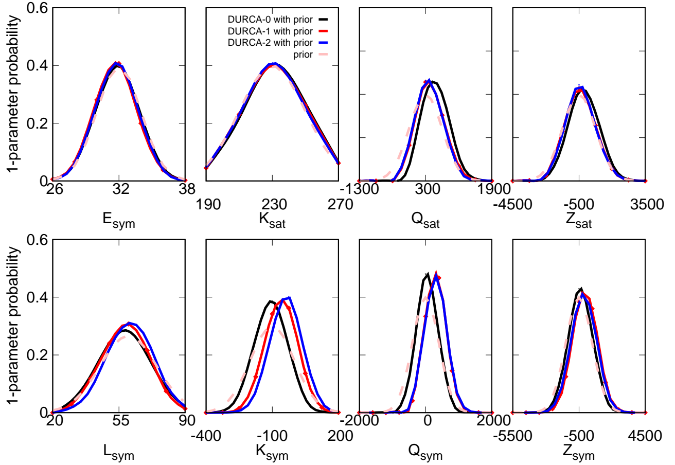
FIG. 4. (Color online) 1-parameter probability distributions p(P_\alpha) . See text for more details.
