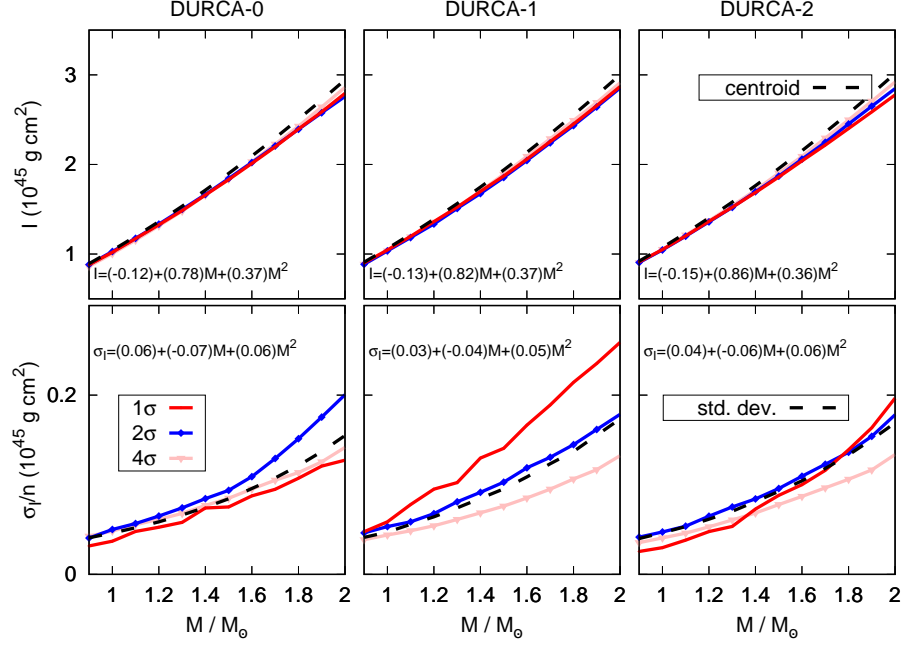
FIG. 12. (Color online) Same as Fig. 11 for the moment of inertia.
