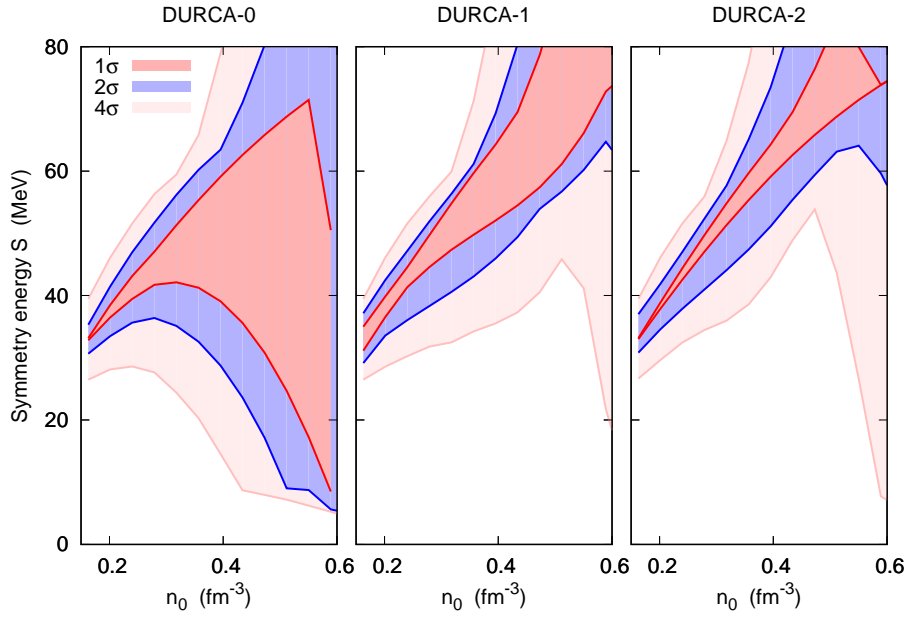
FIG. 17. (Color online) Same as Fig. 15 for the symmetry energy.
