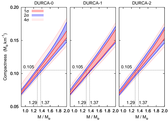
FIG. 10. (Color online) Compactness (M/M_\odot)/(R/km) as a function of the mass for the three hypothesis DURCA-0, 1, 2.
