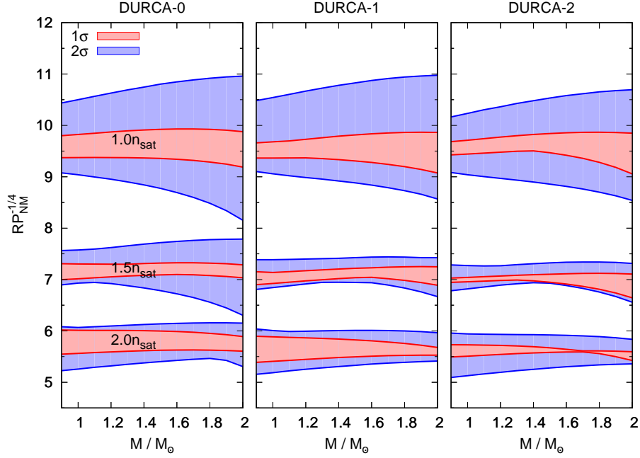
FIG. 14. (Color online) Empirical relation between the pressure (in \text{MeV fm}^{-3} ) and the radius (in km) function of the mass. The pressure is calculated in NM and is defined at 1.0n_{\text{sat}} , 1.5n_{\text{sat}} , or 2.0n_{\text{sat}} as indicated in the plots. We used the same units on the y-axis as in Ref. [25].
