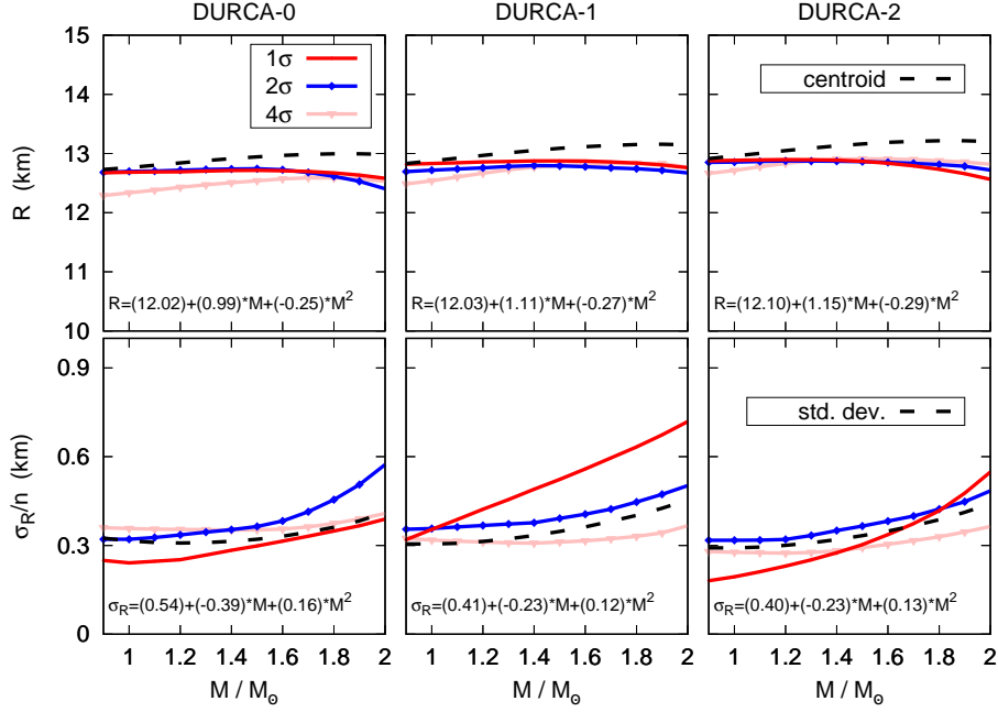
FIG. 11. (Color online) Centroids and standard deviation of the NS radii function of the mass, with DURCA-0, 1, 2.
