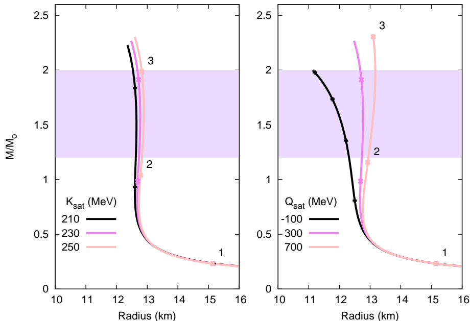
FIG. 2. (Color online) M-R diagram generated with meta-EOS where the isoscalar empirical parameters are varied. See text for more details.
