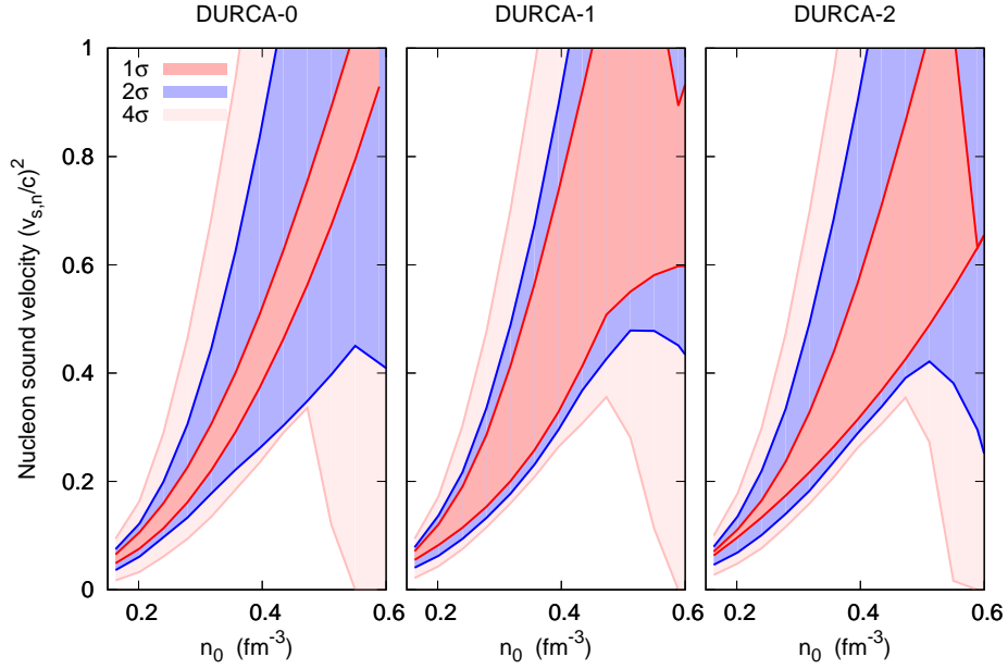
FIG. 20. (Color online) Same as Fig. 15 for the baryon sound velocity.
