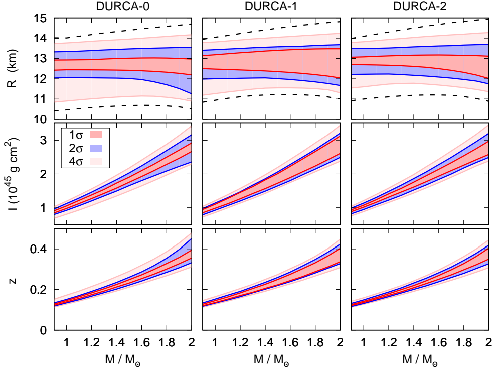
FIG. 8. (Color online) 1\sigma -CL, 2\sigma -CL and 4\sigma -CL domains for the correlation between the total radius R , moment of inertia I and surface redshift z function of the mass M for DURCA-0, 1, and 2 scenarii. The dashed lines on the top panels represent the maximum and minimal values of the radius. See text for discussion.
