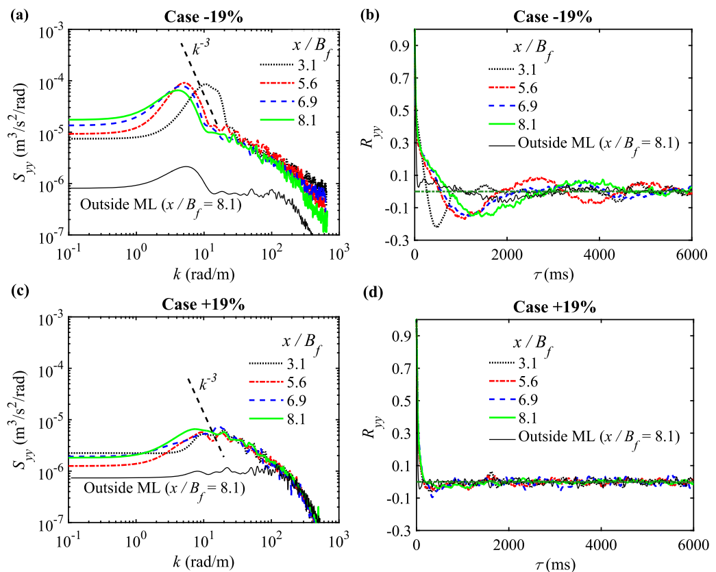
Figure 5. Power density spectra S_{yy} and temporal autocorrelation function R_{yy} of lateral velocity fluctuation v' along the interface ( y/B_f = 1 ) at 40% of the FP flow depth, for 3.1 \leq x/B_f \leq 8.1 . LMFA, relative depth D_r \sim 0.3 : (a, b) case -19\% and (c, d) case +19\% .
