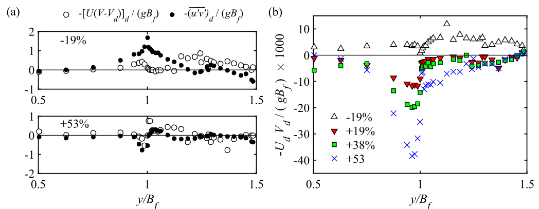
Figure 8. Transverse momentum exchange by (a) the secondary currents -\rho[U(V-V_d)]_d/(gB_f) and turbulent mixing -\rho(u'v')_d/(gB_f) , and by (b) the transverse flow -U_d V_d/(gB_f) . LMFA, nonuniform cases with D_r \sim 0.4 , at x/B_f = 5.6 .
