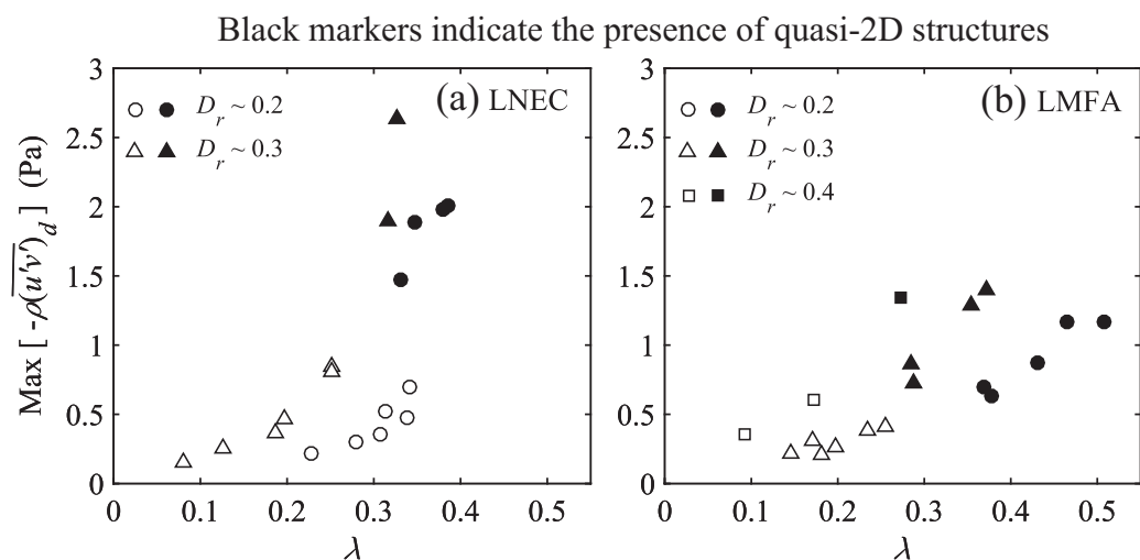
Figure 12. Peak depth-averaged Reynolds-stress \text{Max} [-\rho \overline{(u'v')}_d] across the section at a given downstream position x/B_f as a function of local dimensionless shear \lambda ( x/B_f ), for various relative depths D_r . Measurements at (a) x/B_f = 7.1 and 10.7 at LNEC and (b) x/B_f = 5.6 and 8.1 at LMFA.
