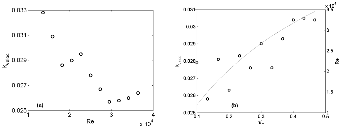
Figure 7. Evolution of k_{veloc} coefficient from Series 2 as a function of Re with fixed values of h/L (a) and from Series 3 as a function of h/L (symbols) with Reynolds numbers (solid line) increasing simultaneously (b).
