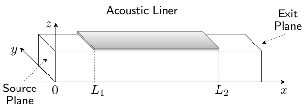
Fig. 1. Sketch of the grazing flow impedance tube
